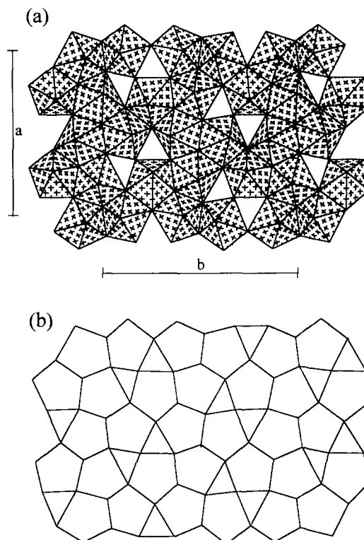
Fig. 4. The sheets of \text{Ur}\phi_5 polyhedra in the structure of schoepite: (a) polyhedral representation; (b) sheet anion-topology. Legend as in Fig. 2.
