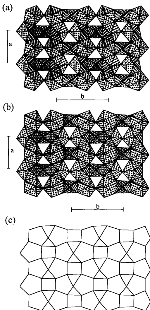
Fig. 3. The sheets of \text{U}\phi_n polyhedra in the structure of ianthinite. Polyhedral representations of the sheets at: (a) z \approx 0.0 and (b) z \approx 0.25 . The sheet anion-topology is shown in (c). Legend as in Fig. 2.
