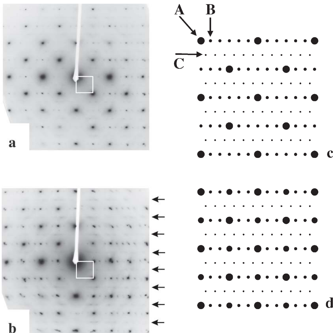
FIG. 5. hk0 electron-diffraction pattern of schwartzembergite: (a) Two-minute exposure showing relatively intense reflections due to the I4/mmm subcell. Rows of very weak B reflections parallel to [010] also are present. Some spots at forbidden ( h + k = \text{odd} ) positions are diffraction spikes from sublattice reflections of the hk1 and hk\bar{1} layers. (b) Three-minute exposure of the same crystallite as in (a). The longer exposure time has allowed strong sublattice reflections from the hk1 and hk\bar{1} layers to be recorded. Rows of B reflections parallel to [010] are evident. Lines of weak spots from C reflections are indicated by arrows. Additional diffraction spots from a second crystallite that is slightly rotated relative to the main one also are present. This second crystallite is probably a piece of the main grain that became detached and rotated. Multi-crystalline patterns often confuse the interpretation of diffraction patterns of these easily cleaved, layered minerals. (c) Schematic diffraction pattern for 3(a). (d) Schematic diffraction pattern for 3(b).
