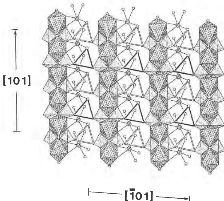
FIG. 3 Linkage of [\text{Cu}(\text{P}_2\text{O}_7)\phi] chains along [\bar{1}01] in wooldridgeite (projected down [010] ); polyhedral shading as in Figure 1, small unshaded circles are (\text{H}_2\text{O}) groups, and \text{Na}-\text{O} bonds are shown as thin lines, the heavily drawn triangles are faces of (\text{Ca}\phi_6) octahedra above the plane of the sheet, and the double-line triangles are faces of (\text{Ca}\phi_6) octahedra below the plane of the sheet.
