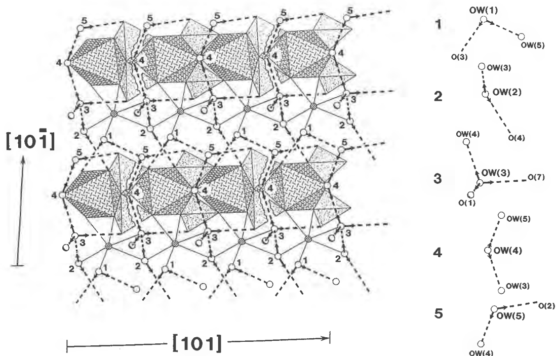
FIG. 6. The structure of woolldridgeite projected down [010] and showing the network of H-bonds; donor \rightarrow acceptor bonds are shown as heavy broken lines. Local details of each (\text{H}_2\text{O}) group are shown to the right of the figure.
