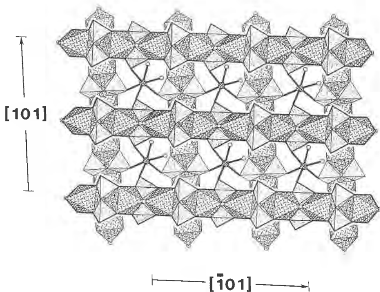
FIG. 4. The relation between adjacent sheets in wooldridgeite, omitting the Na atoms for clarity; polyhedron shading as in Figure 2, and Ca- \phi bonds shown as heavy lines.
