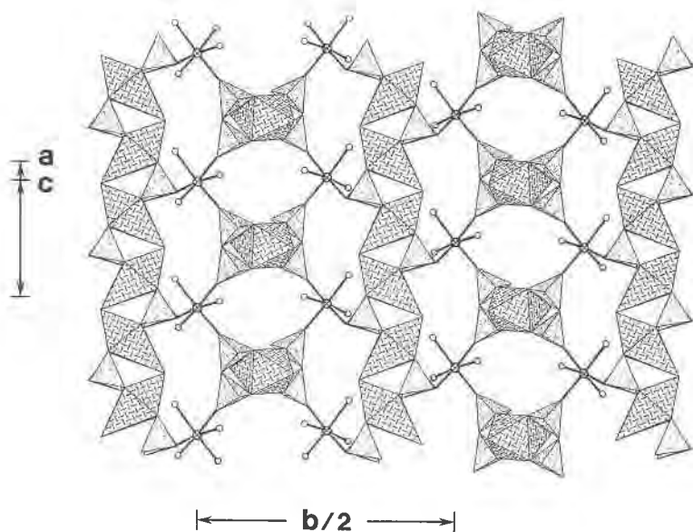
FIG. 5. The structure of wooldridgeite projected onto (101), legend as in Figure 3; Na atoms (omitted for clarity) occur in the interstices between chains adjacent along [101]
