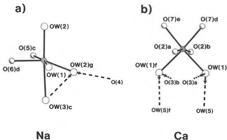
FIG. 1. The coordination of the interstitial-cation sites: (a) Na (diagonal-shaded circles); (b) Ca (cross-hatched circles); highlighted circles are O atoms, larger unshaded circles are ( \text{H}_2\text{O} ) groups, donor \rightarrow H bonds are shown as arrows, H \rightarrow acceptor bonds are shown as broken lines.
