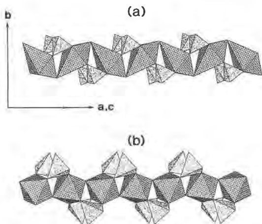
FIG. 2. (a) Perspective view of the [\text{Cu}(\text{P}_2\text{O}_7)\phi] chain in wooldridgeite; (b) perspective view of the type-VI [\text{Al}(\text{PO}_4)_2(\text{OH})] chain in sinkankasite; (\text{PO}_4) tetrahedra are irregularly dot-shaded, and (\text{Cu}\phi_6) octahedra are dash-shaded, and (\text{Al}\phi_6) tetrahedra are cross-shaded.
