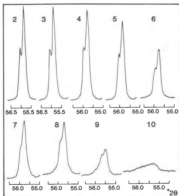
Fig. 4. The 330 X-ray diffraction peak of titanite samples in order of decreasing quality.
