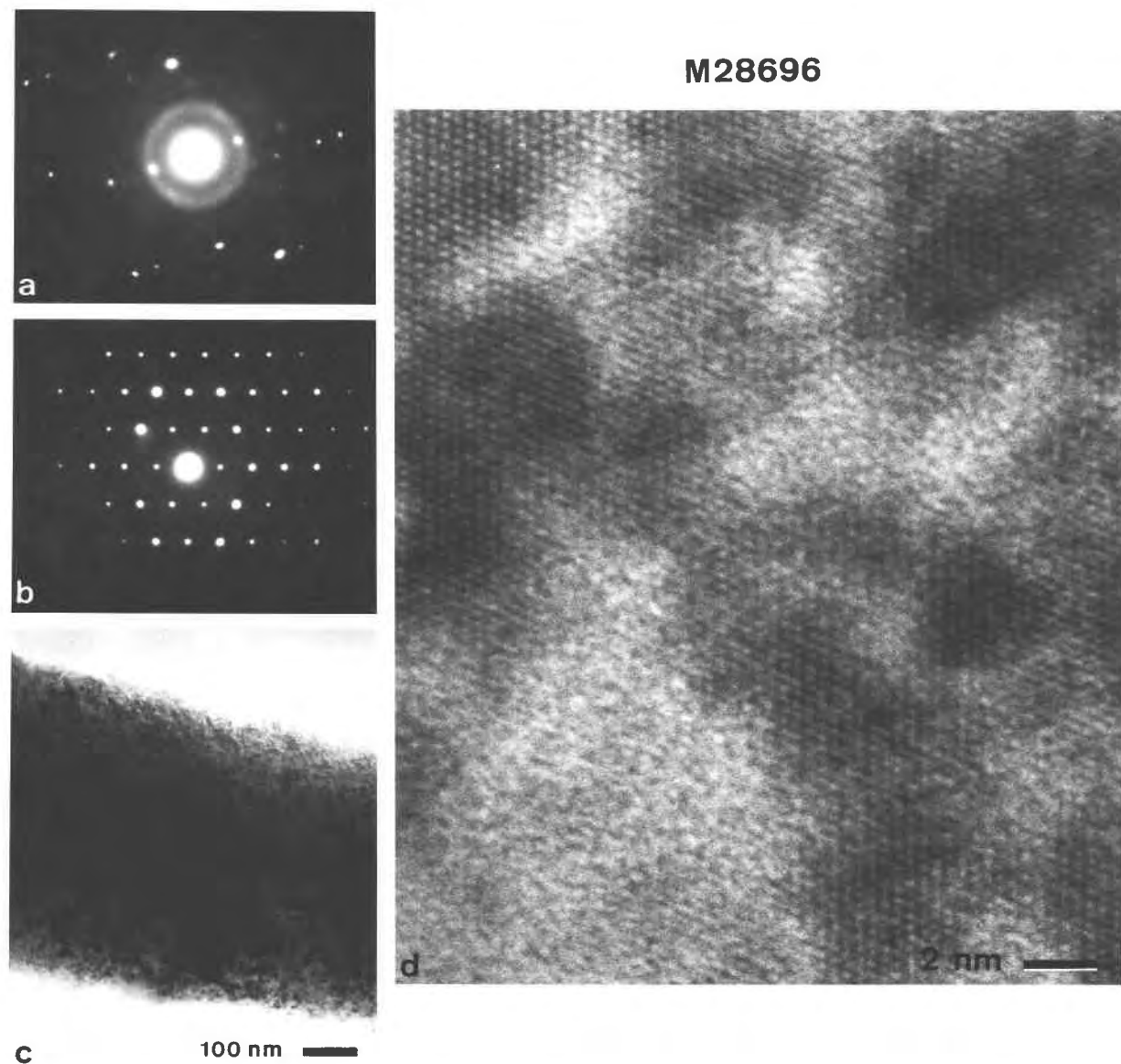
Fig. 16. Cardiff titanite sample: (a) diffraction pattern, tilted and exposed to show the diffuse halo at 3.00 \text{ \AA} ; (b) oriented diffraction pattern ([101] zone) of the grain shown in c, with the diffuse halo still weakly visible; (c) bright-field image showing strong mottled diffraction contrast; and (d) HRTEM image clearly showing coexisting crystalline and aperiodic domains.
