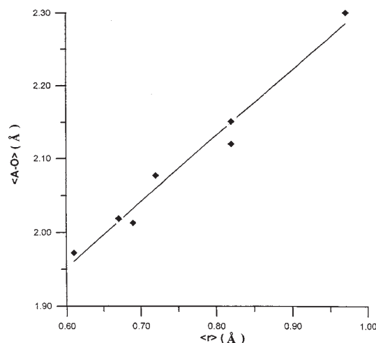
FIG. 3. Variation in \langle A-O \rangle as a function of constituent-cation radius at the A site for Li- and Zn-bearing minerals having the milarite-type structure.
