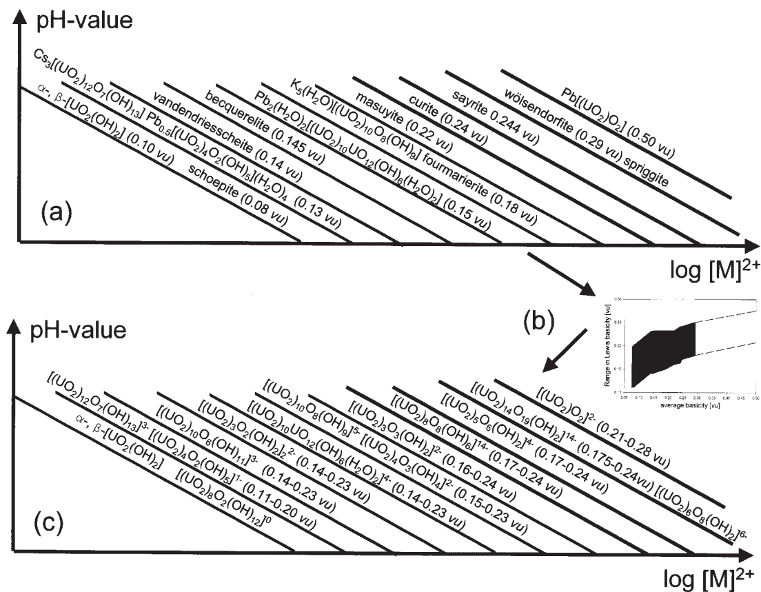
FIG. 9. (a) An activity-activity diagram: pH versus \log [M^{2+}] for selected uranyl-oxide hydroxy-hydrate minerals. The diagram has been calculated without considering different types of interstitial cations (e.g., Pb^{2+} , Ca) or the possible influence of Eh, and stereoactive lone-pair effects are not considered. The corresponding average basicity of the structural unit is given in brackets; (b) the correlation between average basicity and the range in Lewis basicity for all uranyl minerals; (c) the general occurrence of the structural units in the activity-activity diagram with the corresponding ranges in Lewis basicity from Figure 9b.
