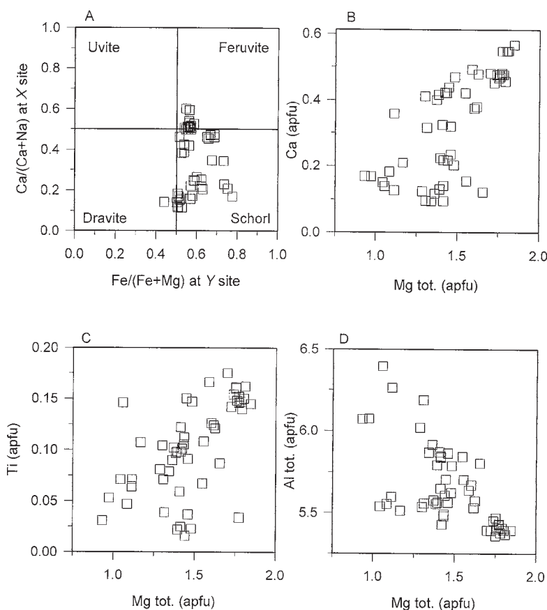
FIG. 2. Group-1 tourmaline compositions from the exocontacts at Tanco. A. \text{Ca}/(\text{Ca} + \text{Na}) at the X site versus \text{Fe}/(\text{Fe} + \text{Mg}) at the Y site. Quadrants are labeled according to the dominant tourmaline end-members. B. Ca versus total Mg (apfu). C. Ti versus total Mg (apfu). D. Total Al versus total Mg (apfu).
