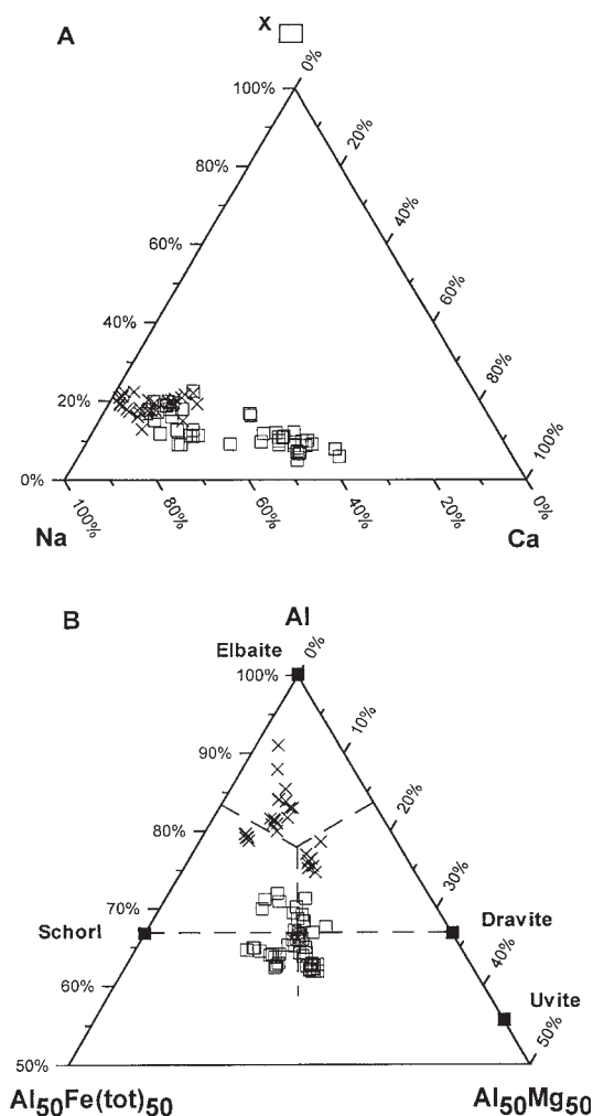
FIG. 1. Tourmaline compositions from the exocontacts at Tanco. A. X□-Na-Ca diagram. B. Al-Fe-Mg diagram. ■: end members; □: group-1 tourmaline; ×: group-2 tourmaline.
