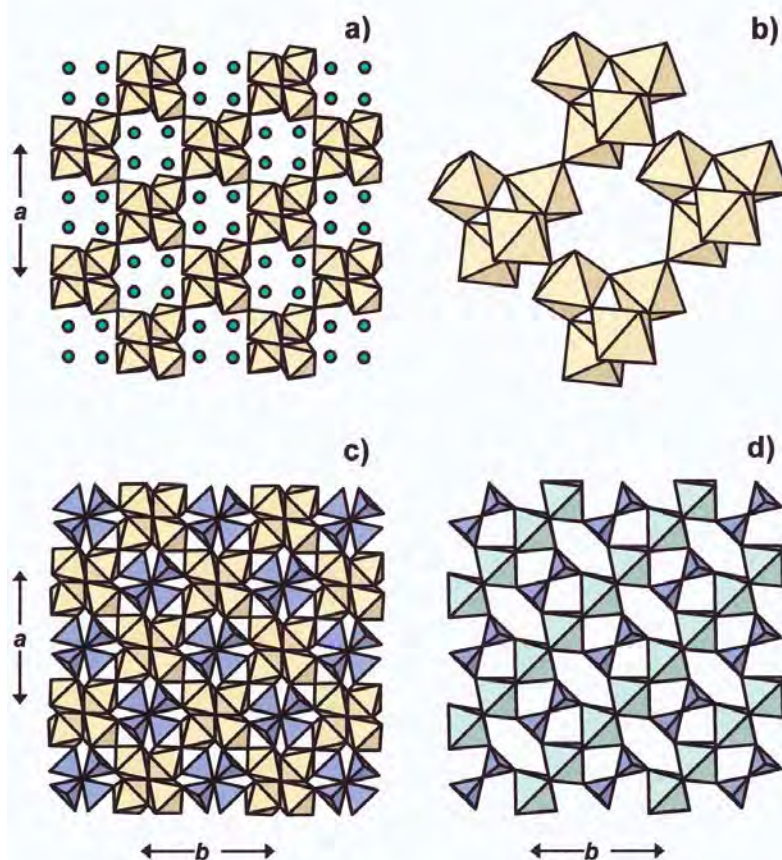
FIG. 1. Fersmanite: (a) the layer formed by the intersection of chains of corner-sharing ( \text{MO}_6 ) octahedra projected onto (001); (b) linkage of four [\text{M}_4\text{O}_{18}] clusters; (c) the layer of corner-sharing ( \text{MO}_6 ) octahedra decorated with [\text{Si}_2\text{O}_7] groups; (d) linkage of \{\text{A}(3,4)\text{O}_6\} octahedra and [\text{Si}_2\text{O}_7] groups. ( \text{MO}_6 ) octahedra are honey-yellow, \text{A}(1) and \text{A}(2) atoms are shown as bright green circles, \{\text{A}(3)\text{O}_6\} and \{\text{A}(4)\text{O}_6\} octahedra are pale green; (\text{SiO}_4) tetrahedra are purple.
