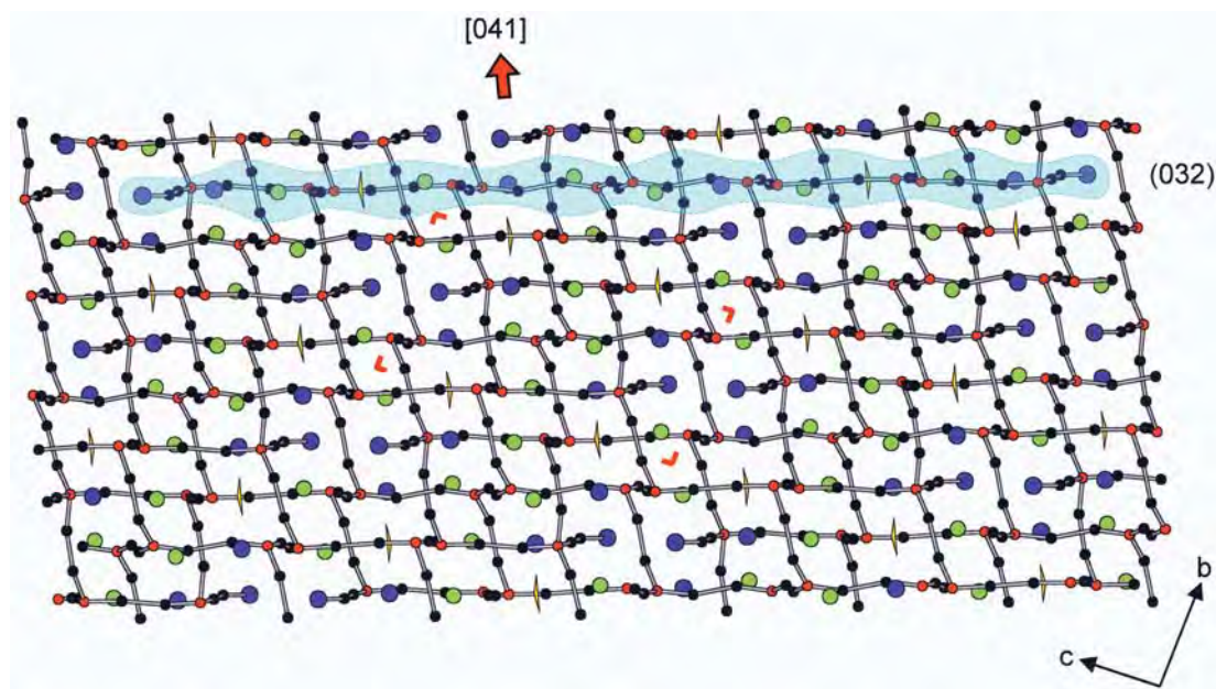
FIG. 3. The crystal structure of vasilyevite viewed down the a axis. Legend as in Figure 1; carbonate groups: yellow triangles, grey lines: strong axial bonds of the [\phi-\text{Hg}-\text{Hg}-\phi] groups. Four red right-angle markers: corners of the unit cell.
