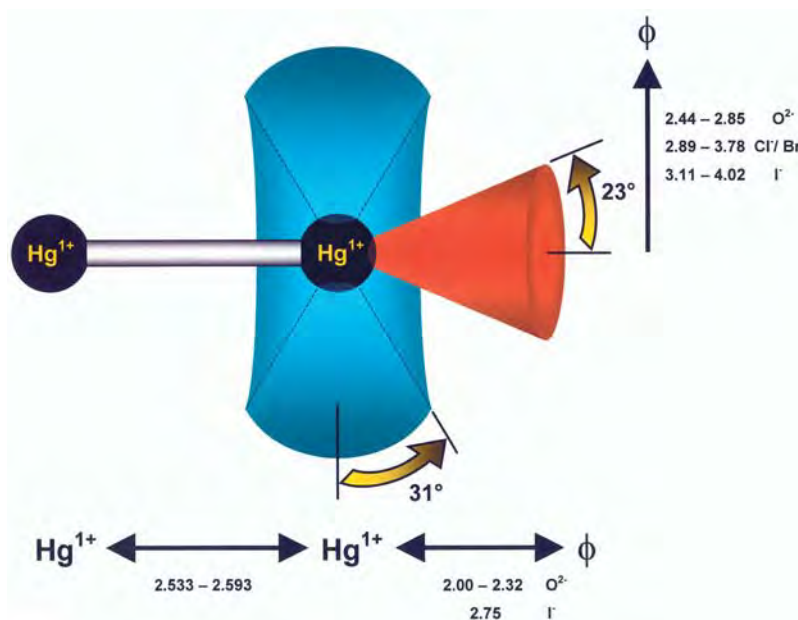
FIG. 2. Stereochemical variation for the eleven [\text{Hg}-\text{Hg}]^{2+} dimers in vasilyevite; orange: axial-bond region, blue: meridional-bond region.
