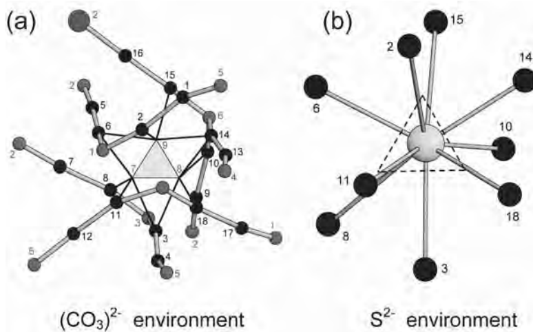
FIG. 5. The environments of the (\text{CO}_3) group (a) and the \text{S}^{2-} anion (b) in vasilyevite. Legend as in Figures 1, 3. Thin black lines: weak bonds from Hg atoms to O atoms of the (\text{CO}_3) group, yellow circle: \text{S}^{2-} atom, dashed triangle: outline of unoccupied (\text{CO}_3) triangle.
