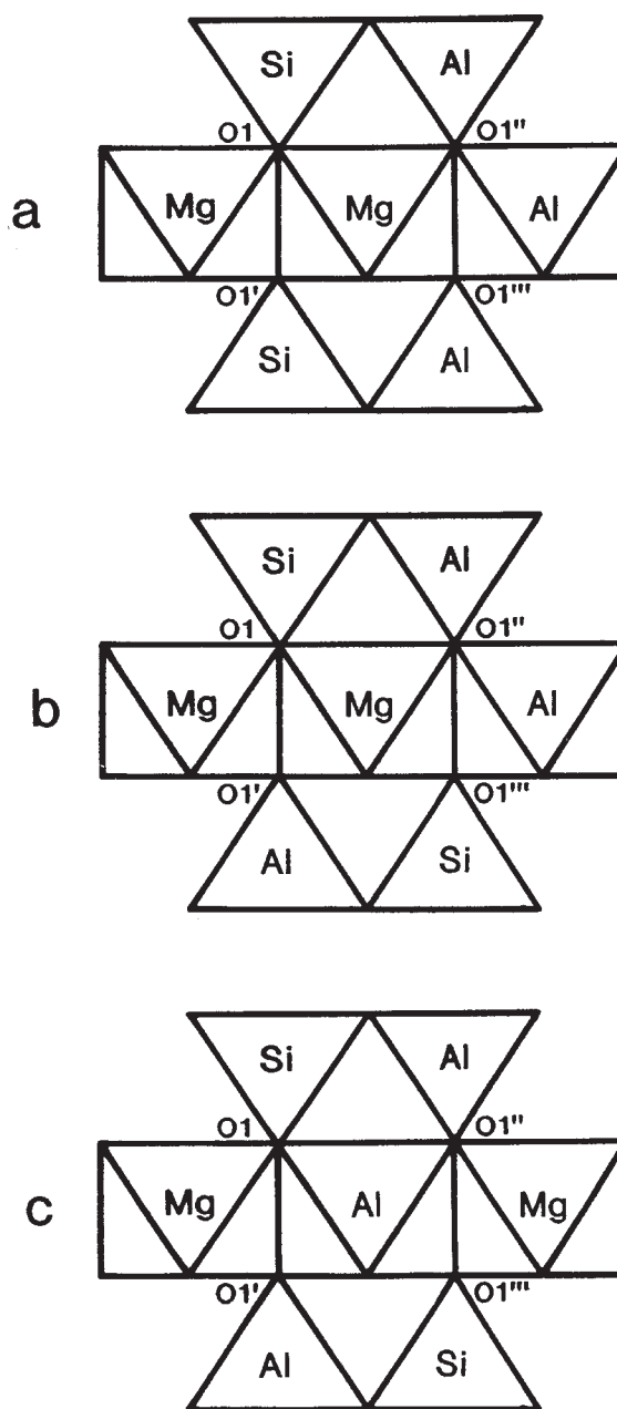
FIGURE 9. Possible short-range arrangements involving Si and Al at the T1 site and Mg and Al at the M2 and M3 sites in the C2/m amphibole structure.
