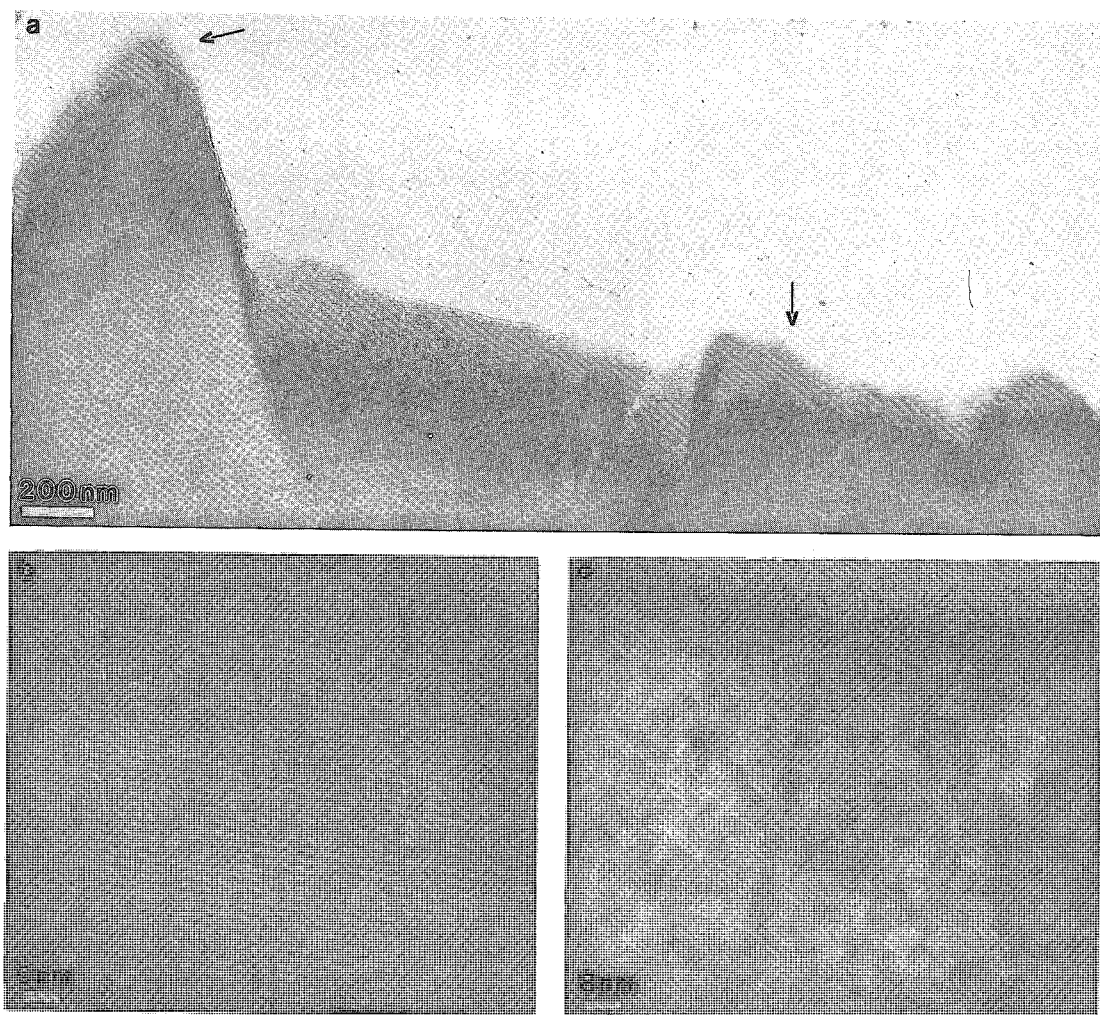
FIG. 7. (a) Electron micrograph of an ion-milled single crystal of V73 in [011] orientation. (b) A lattice image of the area in (a) near the left arrow. (c) A lattice image of the area in (a) near the right arrow. Note the difference in radiation damage between (b) and (c).
