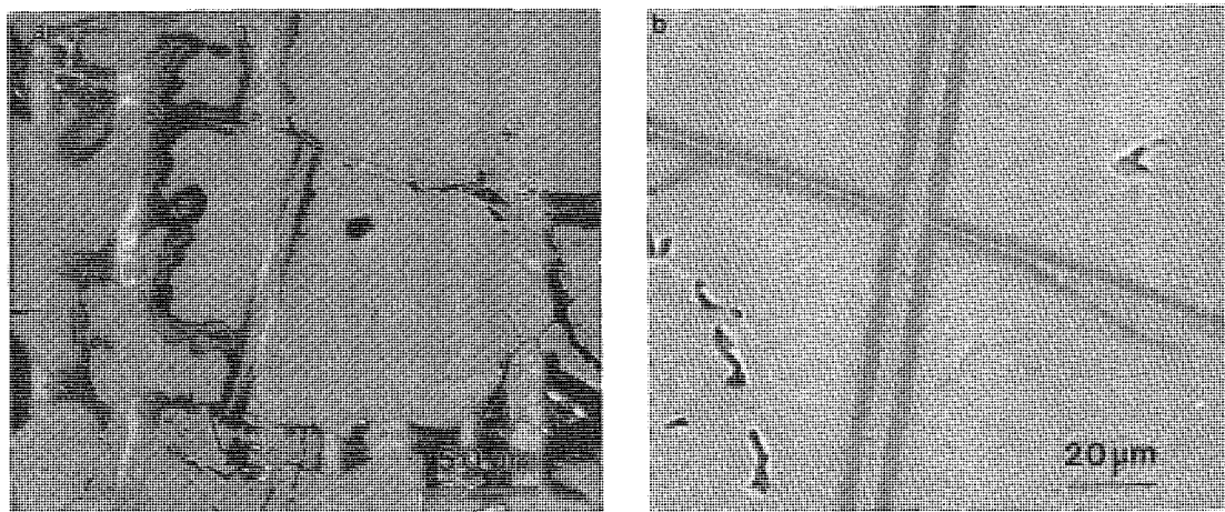
FIG. 3. Back-scattered electron image of V73. Sharply defined linear features have been filled in with titanite, uraninite, and vesuvianite. Their origin is uncertain. (a) A linear zone is offset by later fracturing. (b) Note the symmetrical pattern of alteration.
