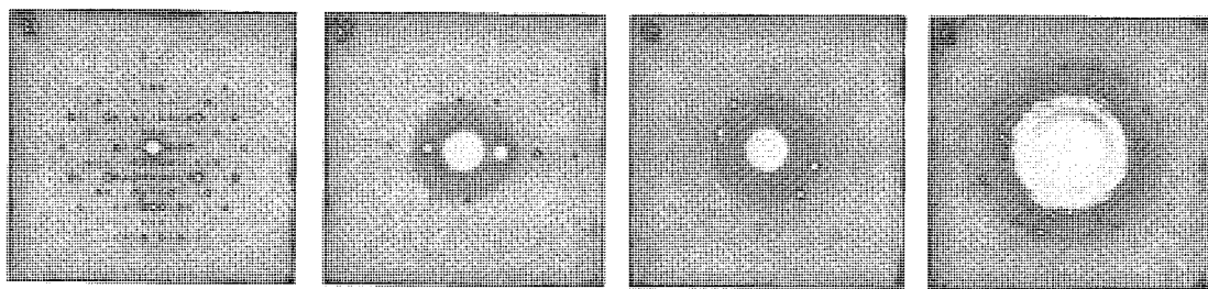
FIG. 6. A series of SAED of V73, with varying amounts of metamictization. (a) [011] ZAP of seemingly undamaged material. (b) An intermediate amount of alpha-recoil damage. (c) An advanced state of alpha-decay damage. (d) A polycrystalline grain with a significant amount of damage as well (note the halo). Ring d -values can be indexed as belonging to vesuvianite.
