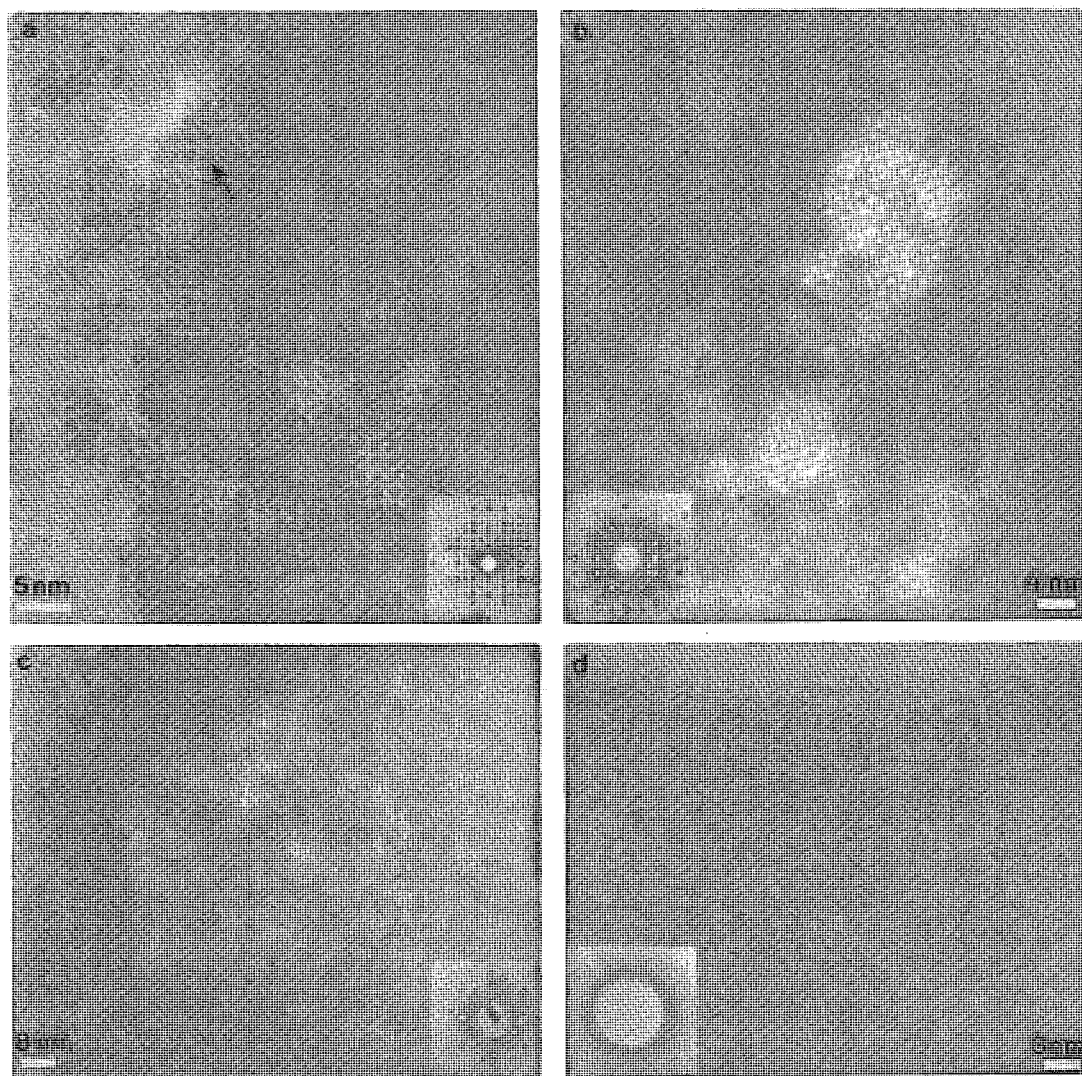
FIG. 5. A series of electron micrographs, each of a different crushed grain of sample V53. (a) A low amount of alpha-recoil damage; SAED is a [001] zone-axis pattern (ZAP). (b) A moderate amount of alpha-recoil damage; [001] ZAP. (c) An advanced state of alpha-decay damage. (d) The fully metamict state.
