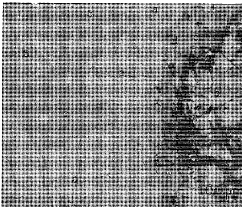
FIG. 2. Back-scattered electron image of V73. Chemical alteration is evident by the areas of different contrast. Regions labeled as a , b , and c correspond to U-poor, U-rich, and altered-rim U-rich compositions (V73-1, V73-2, V73-3, respectively, in Table 1).
