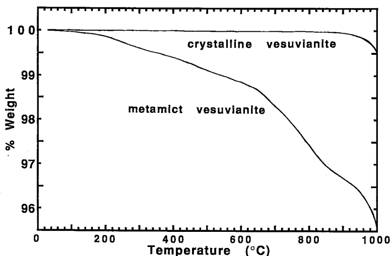
FIG. 9. Thermogravimetric analysis curves for V73 and a sample of crystalline vesuvianite from Phillips, Maine, heated at 10°C/min in flowing argon to 1000°C.
