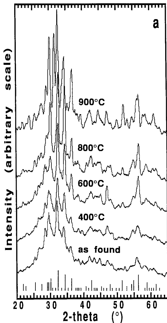
FIG. 8a. Powder XRD pattern (CuK \alpha radiation) of sample V73 as found and annealed in nitrogen (24 hours each) at 400°, 600°, 800° and 900°C. The stick pattern at the bottom shows the peak positions and relative intensities typical of crystalline vesuvianite.
