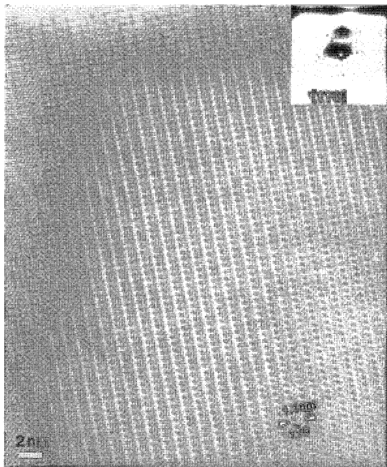
FIG. 4. A high-resolution electron micrograph of nonmetamict vesuvianite in [110] zone-axis orientation.
