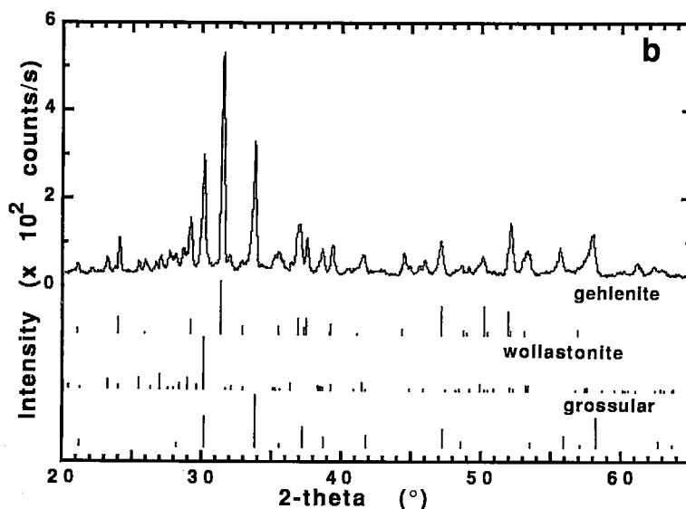
FIG 8b. Powder XRD pattern (CuK \alpha radiation) of sample V73 decomposed at 1000°C (24 hours in nitrogen), with the major products of decomposition shown by stick patterns.
