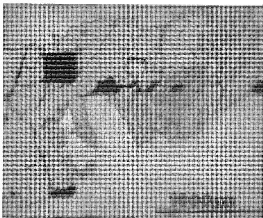
FIG. 1. Back-scattered electron image of V53. Chemical alteration is represented by areas of differing contrast ( i.e. , different atomic mass); the light, medium and dark grey areas each have a different composition, corresponding to compositions V53-1, V53-2 and V53-3, respectively, in Table 1.
