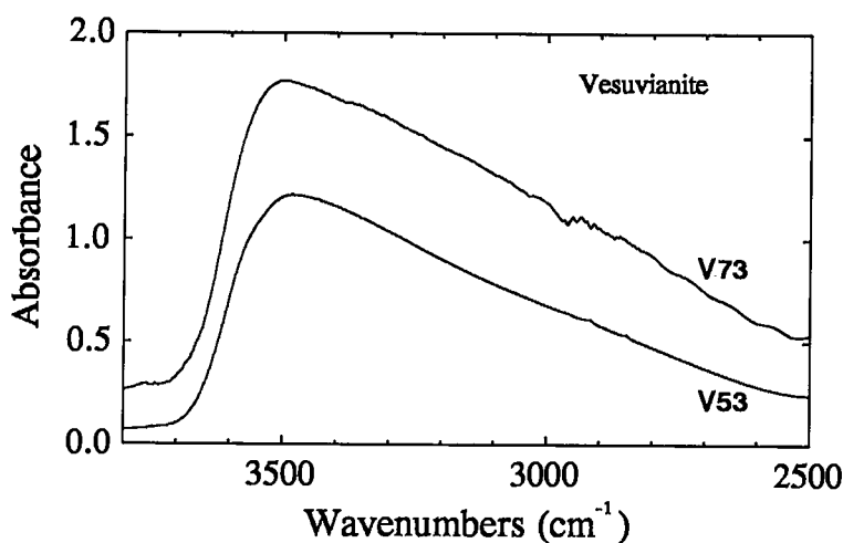
Fig. 11. Single-crystal infrared spectra of V53 and V73 in the principal OH-stretching region. Both spectra show the low-energy tailing absorption common in metamict minerals.
