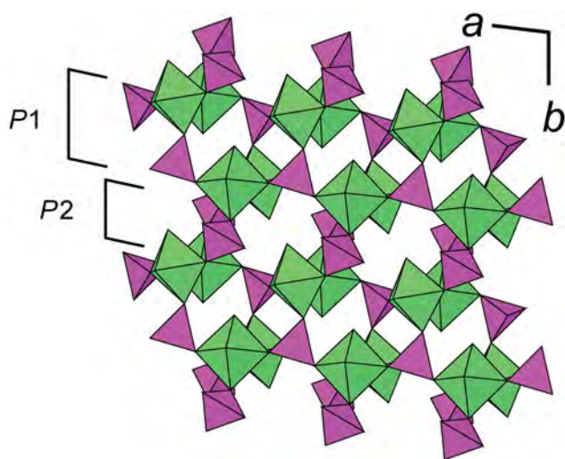
Fig. 4. The slab of [\text{Al}_2\Phi_{11}] dimers and (\text{PO}_4) tetrahedra projected onto (h0l) ; purple = (\text{PO}_4) tetrahedra; green = [\text{Al}_2\text{O}_{10}(\text{OH})] dimers.
