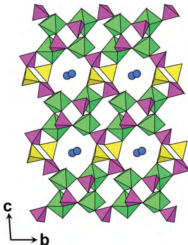
Fig. 5. The structure of brandãoite projected down [100] , showing the slabs of Fig. 4 linked in the c direction by (\text{BeO}_2(\text{OH})\{\text{H}_2\text{O}\}) tetrahedra, with OW5 ( \text{H}_2\text{O} ) groups (blue circles) in the interstices.
