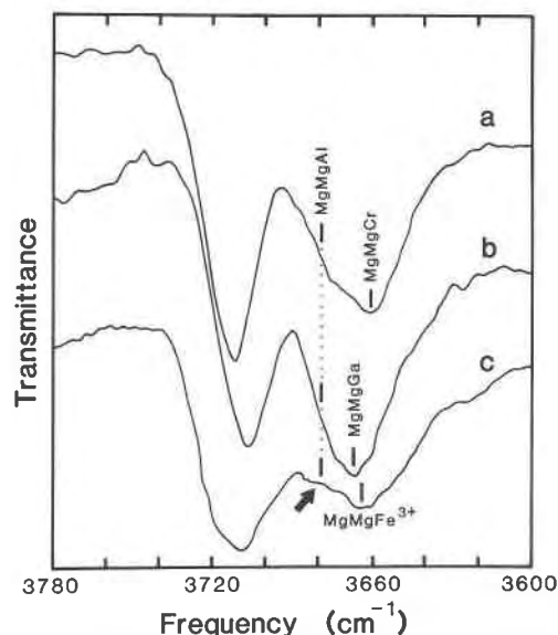
Fig. 4. Infrared spectra of synthetic pargasites and magnesio-hastingsite. Arrow points to MgMgAl bands additional to MgMgCr , MgMgGa , and MgMgFe^{3+} bands. (a) Chromium-pargasite; (b) gallium-pargasite; (c) magnesio-hastingsite (from Semet, 1973).
