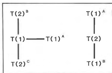
Fig. 9. Next-nearest-neighbor (tetrahedral site) arrangements about the T(1) and T(2) sites in clinoamphiboles.
