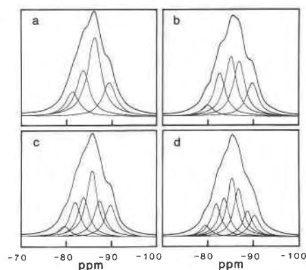
Fig. 8. (a) Four, (b) five, (c) six, and (d) seven peak fits to the ^{29}\text{Si} MAS NMR spectrum of pargasite. Calculated spectrum is shown; experimental envelope shown in Fig. 7b.
