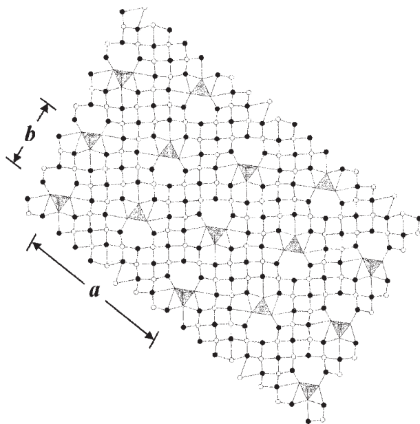
FIGURE 2. The {001} PbO-SO 4 sheet in symesite, showing the ordering pattern of Pb and S; Pb atoms are black circles, O atoms are white circles, sulfate groups are gray tetrahedra. The apical atoms of SO 4 tetrahedra in adjacent (200) rows point in opposite directions; note the juxtaposition of SO 4 tetrahedra and oxygen vacancies.
