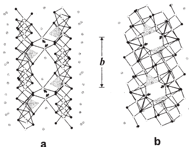
FIGURE 4. The structure of symesite viewed (a) parallel to, and (b) perpendicular to, the PbO and Cl sheets. Orientation (b) is obtained by rotating (a) 90° to the left about the b axis. Pb atoms are black circles, Cl atoms are gray circles, O atoms are white circles, SO 4 groups are gray tetrahedra; only Pb-O bonds are shown for clarity. The O12 atoms of H 2 O groups in the Cl layer are indicated by arrows. O2-O12 distances are 2.80(7) and 3.07(6) Å with inter-oxygen angles of 91(2)°.
