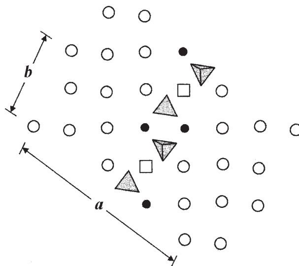
FIGURE 3. The {001} Cl-H 2 O layer in symesite. Eight of eleven anion sites are occupied by Cl (white circles), two by O12 of H 2 O groups (small black circles), and there is one vacant site (square). The Cl and O12 atoms are approximately coplanar. The apical O2 atoms of the SO 4 tetrahedra lie midway between Cl and PbO sheets. Upward-pointing tetrahedra are in the PbO sheet below the Cl layer, and downward-pointing tetrahedra are in the PbO sheet above the anion layer.
