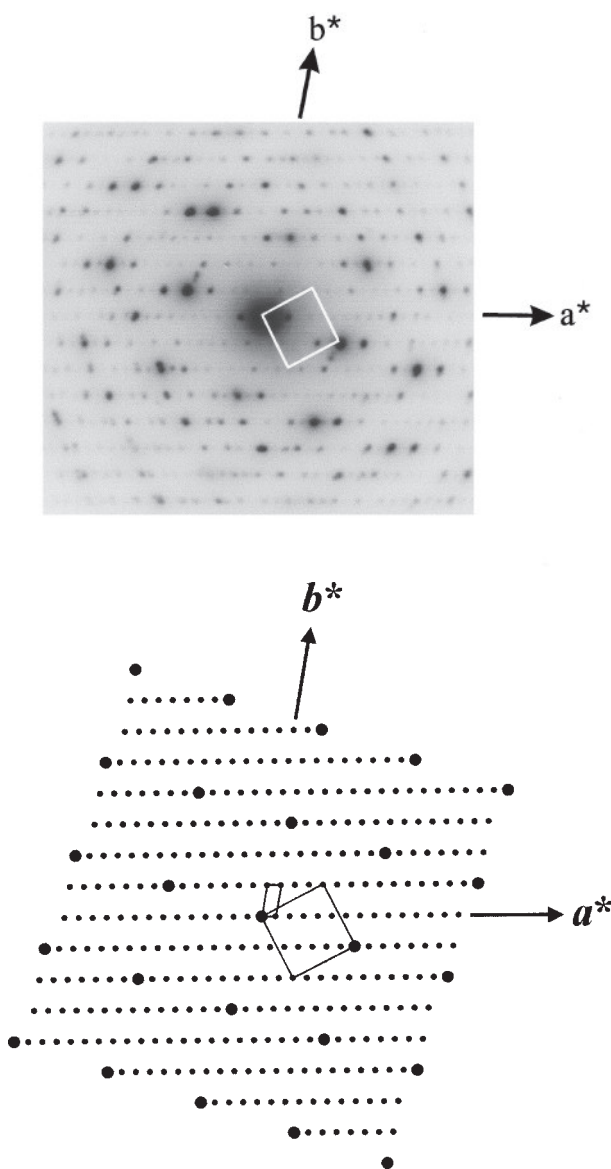
FIGURE 1. (a) Electron-diffraction pattern of symesite with the beam normal to the {001} cleavage and the PbO-SO 4 sheets. In addition to the relatively strong substructure reflections ( h + k = 2n ), there are rows of many weak, sharp superstructure reflections. A reciprocal 0.25/\text{\AA} \times 0.25/\text{\AA} subcell is indicated, and a^* and b^* directions for the B\bar{1} supercell are shown. (b) Reciprocal subcell and B\bar{1} supercells are indicated.
