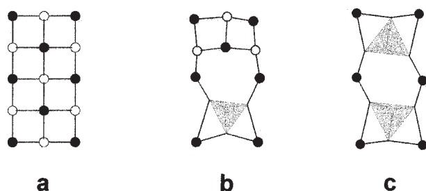
FIGURE 6. The local structure around the SO 4 tetrahedron in symesite (b) compared with litharge (a) and the VO 4 tetrahedra in komatite (c).
