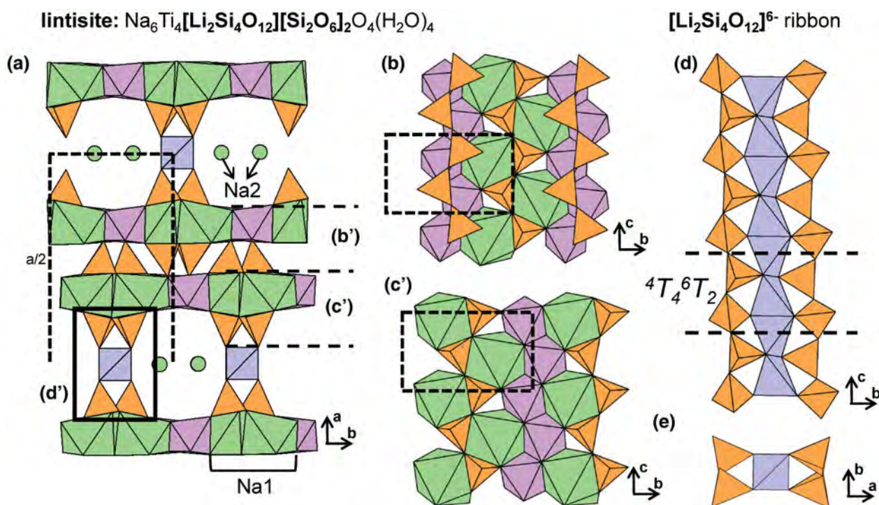
Fig. 6. The structure of linitisite projected (a) along the c -axis, (b, c) onto (100), and the [\text{Li}_2\text{Si}_4\text{O}_{12}]^{6-} ribbon of [\text{SiO}_4]^{4-} and [\text{LiO}_4]^{7-} tetrahedra projected (d) onto (100) and (e) along the c -axis. Fine dashed black lines outline the unit cell which is halved along the a -axis in (a). The H atoms associated ( \text{H}_2\text{O} ) groups have been omitted for clarity.
