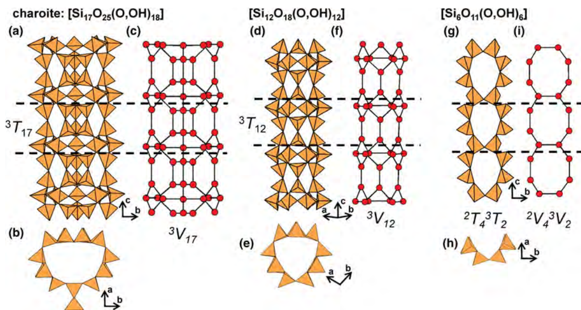
Fig. 52. (a, b, c) Tetrahedral representation of the 3T_{17} tube in charoite projected (a) onto (100), (b) along the c -axis and (c) a ball-and-stick representation of this tube. (d, e, f) the 3T_{12} tube in charoite projected (d) orthogonal to the c -axis, (e) along the c -axis and (f) a ball-and-stick representation of this tube. (g, h, i) the 2T_4^3T_2 ribbon in charoite projected (g) onto (100), (h) along the c -axis and (i) a ball-and-stick representation of this ribbon. Dashed black lines outline the geometrical and topological repeat unit of the tube or ribbon.
