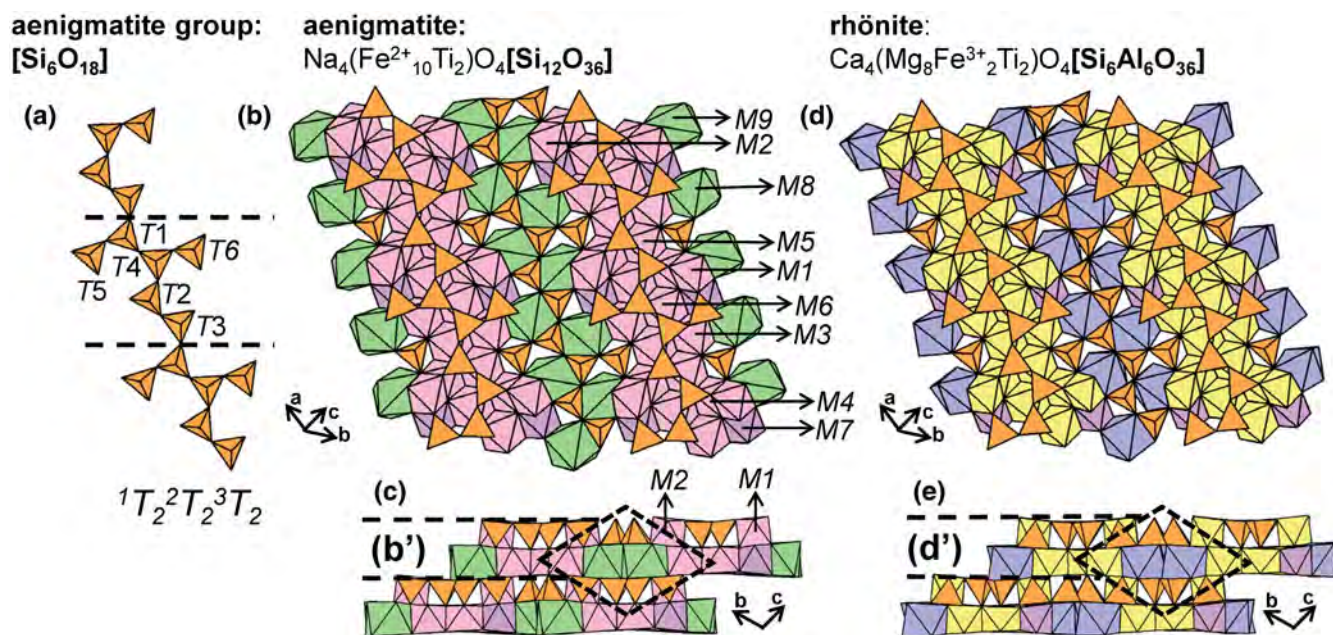
Fig. 97. (a) Tetrahedral representation of the chain in aenigmatite-group minerals. The structure of (b, c) aenigmatite and (d, e) rhönite projected (b, d) orthogonal to the a -axis and (c, e) along the a -axis. The M -site labelling for aenigmatite is applicable to rhönite . Dashed black lines outline the repeat unit of the chain and fine dashed black lines outline the unit cell.
