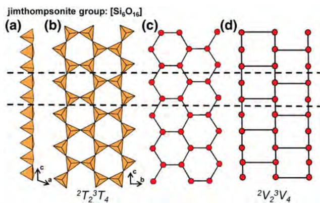
Fig. 65. (a, b) Tetrahedral representations of the 2T_2^3T_4 ribbon in jimthompsonite projected (a) orthogonal to the c -axis, (b) onto (100), (c) a ball-and-stick and (d) a graphical representation of the ribbon. Dashed black lines outline the geometrical and topological repeat unit of the ribbon.
