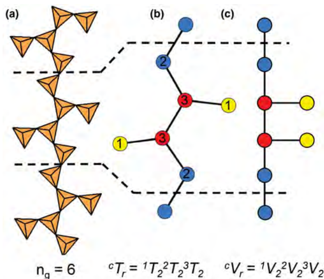
Fig. 2. (a) Tetrahedral, (b) ball-and-stick and (c) graphical representations of the chain in sapphirine-supergroup minerals viewed orthogonal to the c -axis. Each tetrahedron in (a) is represented by a point (ball) in (b) and a vertex in (c), and all linkages between tetrahedra in (a) are represented by lines (sticks) in (b) and edges in (c) that connect each ball or vertex. Red, blue and yellow points (circles) represent 3-, 2- and 1-connected vertices. Dashed black lines show the geometrical repeat unit in (a) and (b) and the topological repeat unit in (c).
