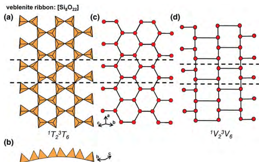
Fig. 60. (a, b) Tetrahedral representations of the 1T_2^3T_6 ribbon in veblenite projected (a) orthogonal to the a -axis, (b) along the a -axis, (c) a ball-and-stick and (d) a graphical representation of the ribbon. Dashed black lines outline the geometrical and topological repeat unit of the ribbon.
