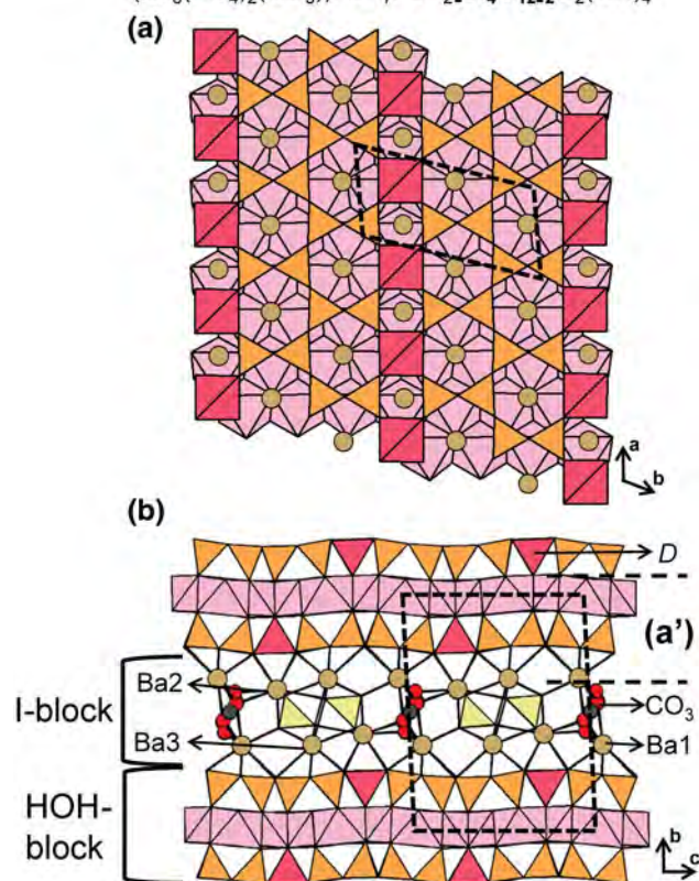
Fig. 57. The structure of devitoite highlighting the (a) H - and O -sheet projected onto (001) and the (b) HOH -block and I -block viewed along the a -axis. In (b), the C and O atoms of the (\text{CO}_3) groups are shown as dark grey and red circles, respectively. The I -block, [\text{PO}_4] groups are shown as yellow polyhedra and [\text{Si}]^{3+} -polyhedra are shown in dark pink to differentiate them from \text{Fe}^{2+} -octahedra. Fine dashed black lines outline the unit cell and H atoms associated with (\text{OH})^- groups are omitted for clarity.
