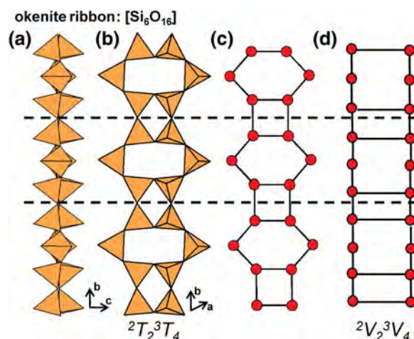
Fig. 67. (a, b) Tetrahedral representations of the 2T_2^3T_4 ribbon in okenite projected (a) onto (100), (b) onto (001), (c) a ball-and-stick and (d) a graphical representation of the ribbon. Dashed black lines outline the geometrical and topological repeat unit of the ribbon.
