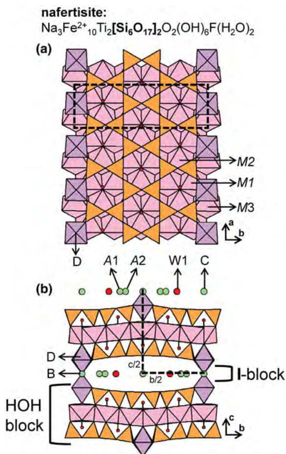
Fig. 59. The structure of nafertisite highlighting the (a) H - and O -sheets projected onto (001) and the (b) HOH-block and I-block viewed along the a -axis. The H atoms associated with (\text{OH})^- groups linked to octahedra of the O -sheet are shown as small red circles, (\text{H}_2\text{O}) groups (W1) are shown as larger red circles and I-block cations are shown as green circles. Fine dashed black lines outline the unit cell which is halved along the c - and b -axes in (b).
