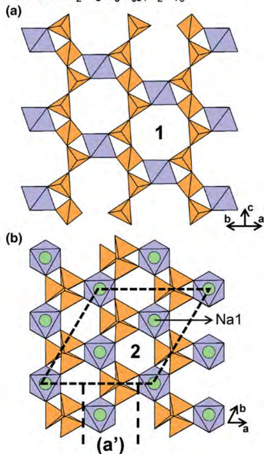
Fig. 15. The structure of hilairite projected (a) orthogonal to the c -axis and (b) along the c -axis. Channel 1 in (a) is occupied by Na1, Na2 and (H 2 O) groups and channel 2 in (b) is occupied by Na2 and (H 2 O) groups. The (H 2 O) groups, Na1 and Na2 in (a) and (H 2 O) groups and Na2 in (b) have been omitted for clarity. Fine dashed black lines outline the unit cell.
