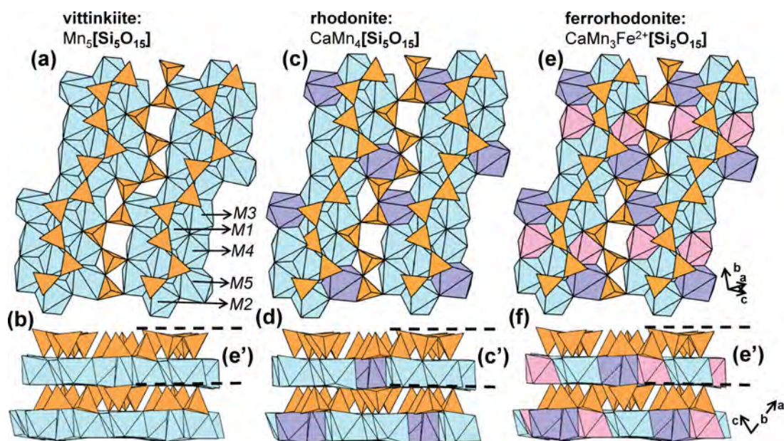
Fig. 26. The structure of (a, b) vittinkiite , (c, d) rhodonite and (e, f) ferrorhodonite viewed (a, c, e) orthogonal to [110] and (b, d, f) along [110] . M-site labels in (a) are also applicable to (c) and (e).
