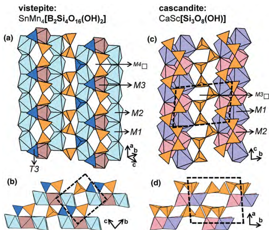
Fig. 14. The structure of vistepite viewed (a) orthogonal to the a -axis and (b) along the a -axis, {}^2T_3[\text{BO}_4] tetrahedra are shown in dark blue. The structure of cascandite projected (c) onto (100) and (d) along the c -axis. Fine dashed black lines outline the unit cell and H atoms associated with (\text{OH})^- groups have been omitted for clarity.
