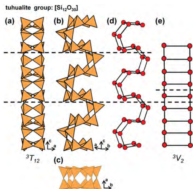
Fig. 46. (a, b, c) Tetrahedral representation of the ^3T_{12} ribbon in tuhualite projected (a) onto (010), (b) orthogonal to the c -axis, (c) along the c -axis, (d) a ball-and-stick and (e) a graphical representation of the ribbon. Dashed black lines outline the geometrical and topological repeat unit of the ribbon.
