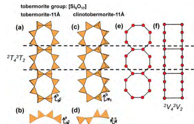
Fig. 75. (a, b, c) Tetrahedral representations of the {}^2T_4 {}^3T_2 ribbon in (a, b) tobermorite-11Å and (c, d) clinotobermorite-11Å projected (a, c) onto (100) and (b, d) along the b -axis. (e) a ball-and-stick and (f) a graphical representation of the ribbon. Dashed black lines outline the geometrical and topological repeat unit of the ribbon.
