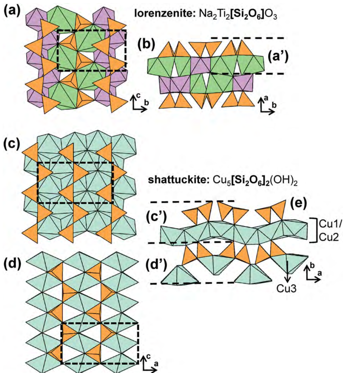
Fig. 8. The structure of lorezenite projected (a) onto (100) and (b) along the c -axis. The structure of shattuckite projected (c, d) onto (010) and (e) along the c -axis. Fine dashed black lines outline the unit cell and H atoms associated with (OH) − groups have been omitted for clarity.
