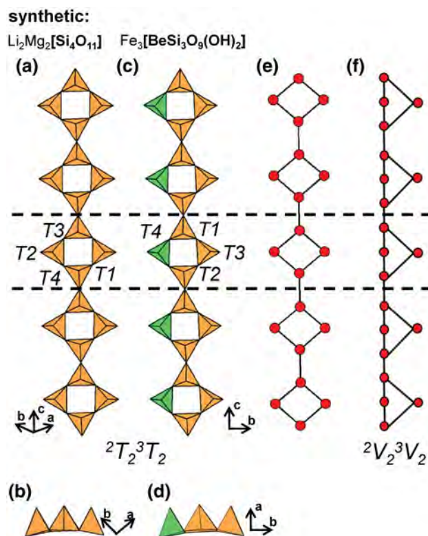
Fig. 64. Tetrahedral representations of the {}^2T_2{}^3T_2 chains in (a, b) synthetic Li_2Mg_2[Si_4O_{11}] and (c, d) Fe_3[BeSi_3O_9(OH)_2] projected (a) orthogonal to the c -axis, (b) along the c -axis, (c) onto (100), (d) along the c -axis, (e) a ball-and-stick and (f) a graphical representation of the both chains. The T4 site in synthetic Fe_3[BeSi_3O_9(OH)_2] is occupied by Be^{2+} and is shown as a dark green tetrahedron. Dashed black lines outline the geometrical and topological repeat unit of the chain.
