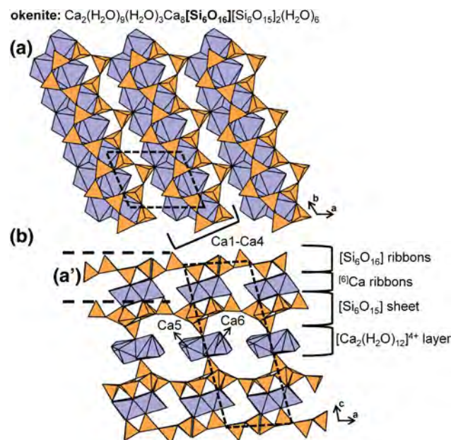
Fig. 68. The structure of okenite projected (a) onto (001) and (b) along the b -axis. Here, layers that contain [\text{Si}_6\text{O}_{16}]^{8-} ribbons, [\text{Si}_6\text{O}_{15}]^{6-} sheets and [\text{Ca}_2(\text{H}_2\text{O})_{12}]^{4+} dimers are labelled. Fine dashed black lines outline the unit cell and H atoms associated with (\text{H}_2\text{O}) groups are omitted for clarity.
