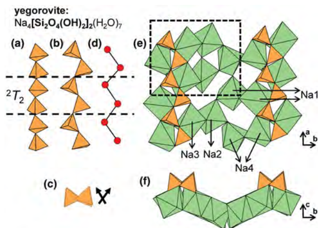
Fig. 9. (a, b, c) Tetrahedral representations of the ^2T_2 chain in yegorovite where both tetrahedra in the geometrical repeat unit point in oblique directions, and (d) a ball-and-stick representation of the chain. The structure of yegorovite projected (e) onto (001) and (f) along the a -axis. Fine dashed black lines outline the unit cell and H atoms associated with (OH) ^- and (H _2 O) groups have been omitted for clarity.
