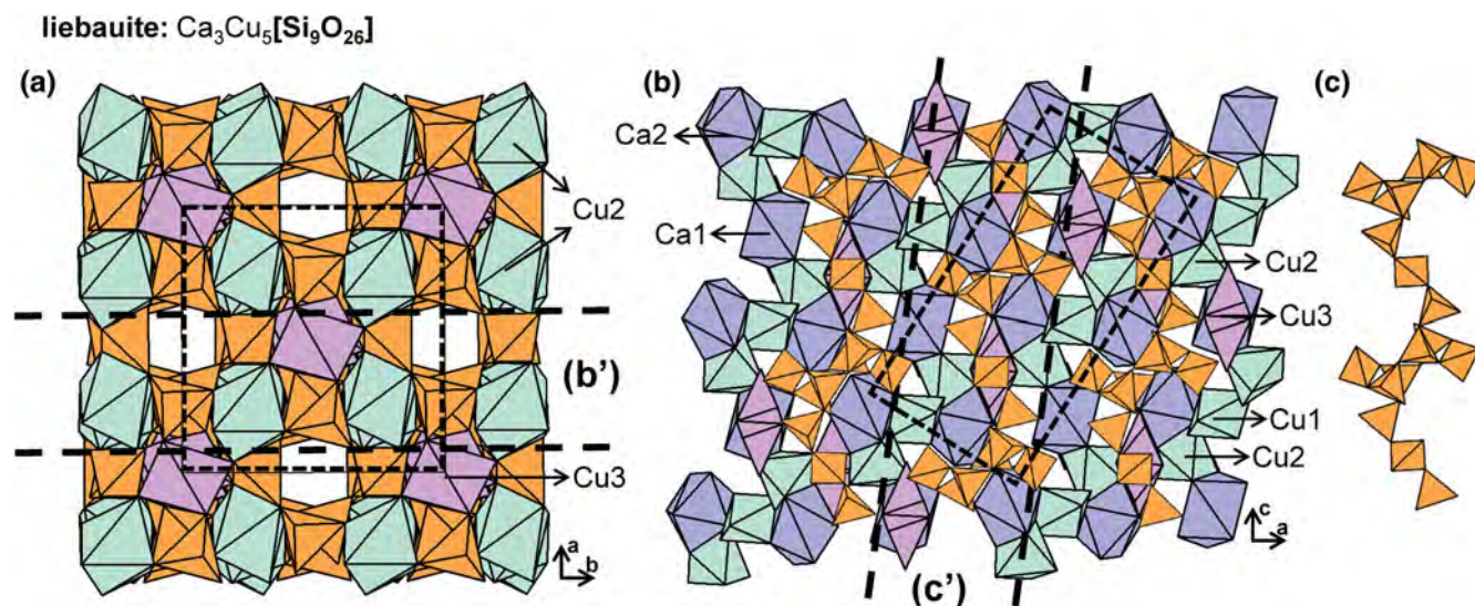
Fig. 89. The structure of liebauite projected (a) along the c -axis, (b) onto (010) and (c) an isolated {}^2T_4{}^3T_2{}^4T_2 chain viewed orthogonal to [101] . For clarity, \text{Cu}^{2+} -octahedra are teal-green and (\text{CuO})_6^{8-} -polyhedra are violet. Fine dashed black lines outline the unit cell.
