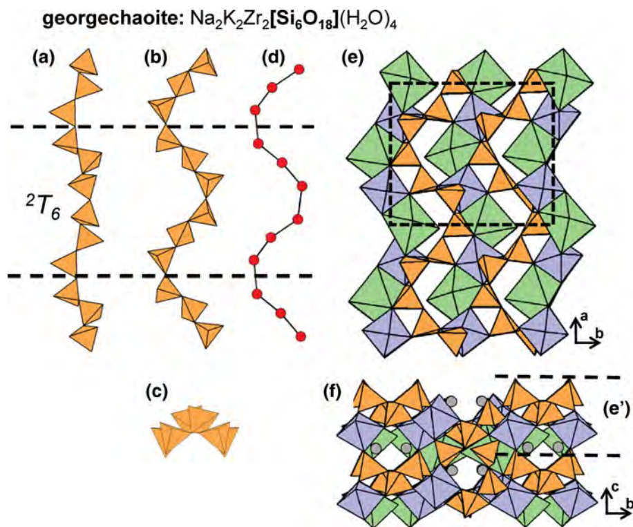
Fig. 30. (a, b, c) Tetrahedral representations of the ^2T_6 chain in georgechaoite and (d) a ball-and-stick representation of the chain. The structure of georgechaoite projected (e) onto (001) and (f) along the a -axis. Dashed black lines outline the geometrical repeat unit of the chain and fine dashed black lines outline the unit cell. The H atoms associated ( \text{H}_2\text{O} ) groups have been omitted for clarity.
