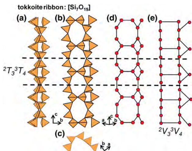
Fig. 71. (a, b, c) Tetrahedral representations of the 2T_3^3T_4 ribbon in tokkoite projected (a) onto (100), (b) orthogonal to the c -axis, (c) along the c -axis, (d) a ball-and-stick and (e) a graphical representation of the ribbon. Dashed black lines outline the geometrical and topological repeat unit of the ribbon.
