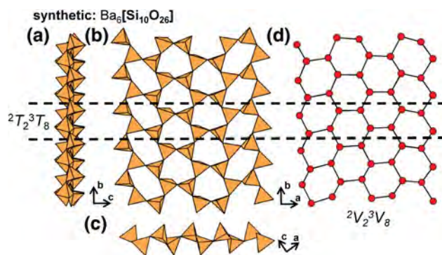
Fig. 70. (a, b, c) Tetrahedral representations of the {}^2T_2^3T_8 ribbon in synthetic Ba_6[Si_{10}O_{26}] projected (a) onto (100), (b) onto (001), (c) along the b-axis and (d) a ball-and-stick (graphical) representation of the ribbon. Dashed black lines outline the geometrical and topological repeat unit of the ribbon.
