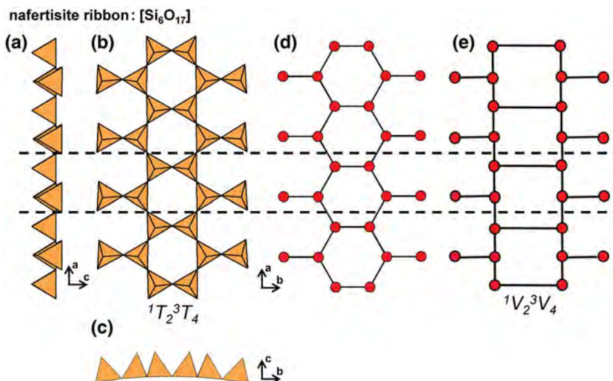
Fig. 58. (a, b, c) Tetrahedral representations of the ^1T_2^3T_4 ribbon in nafertisite projected (a) onto (010), (b) onto (001), (c) along the a -axis, (d) a ball-and-stick and (e) a graphical representation of the ribbon. Dashed black lines outline the geometrical and topological repeat unit of the ribbon.
