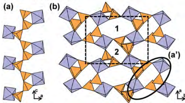
Fig. 16. The structure of umbite projected (a) onto (010) and (b) along the c -axis. In (b), channel 1 is occupied by K2 and (H 2 O) groups and channel 2 is occupied by K1. The (H 2 O) groups, K1 and K2 atoms have been omitted for clarity. Fine dashed black lines outline the unit cell.
