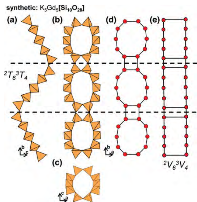
Fig. 86. (a, b, c) Tetrahedral representations of the {}^2T_6{}^3T_4 ribbon in synthetic \text{K}_5\text{Gd}_5[\text{Si}_{10}\text{O}_{28}] projected (a) onto (100), (b) onto (001), (c) along the b -axis, (d) a ball-and-stick and (e) a graphical representation of the ribbon. Dashed black lines outline the geometrical and topological repeat unit of the ribbon.
