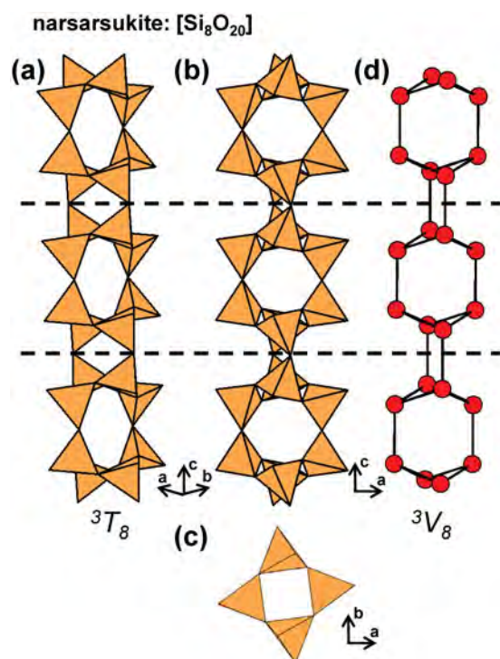
Fig. 44. (a, b, c) Tetrahedral representation of the ^3T_8 tube in narsarsukite projected (a) orthogonal to the c -axis, (b) onto (010), (c) along the c -axis and (d) a ball-and-stick (graphical) representation of the tube. Dashed black lines outline the geometrical and topological repeat unit of the tube.
