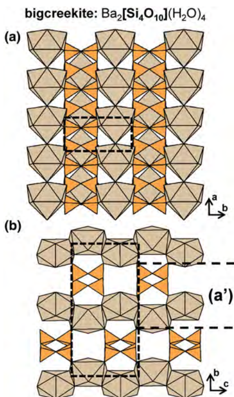
Fig. 37. The structure of bigcreekite projected (a) onto (001) and (b) along the a -axis. Fine dashed black lines outline the unit cell and H atoms associated with ( \text{H}_2\text{O} ) groups have been omitted for clarity.
