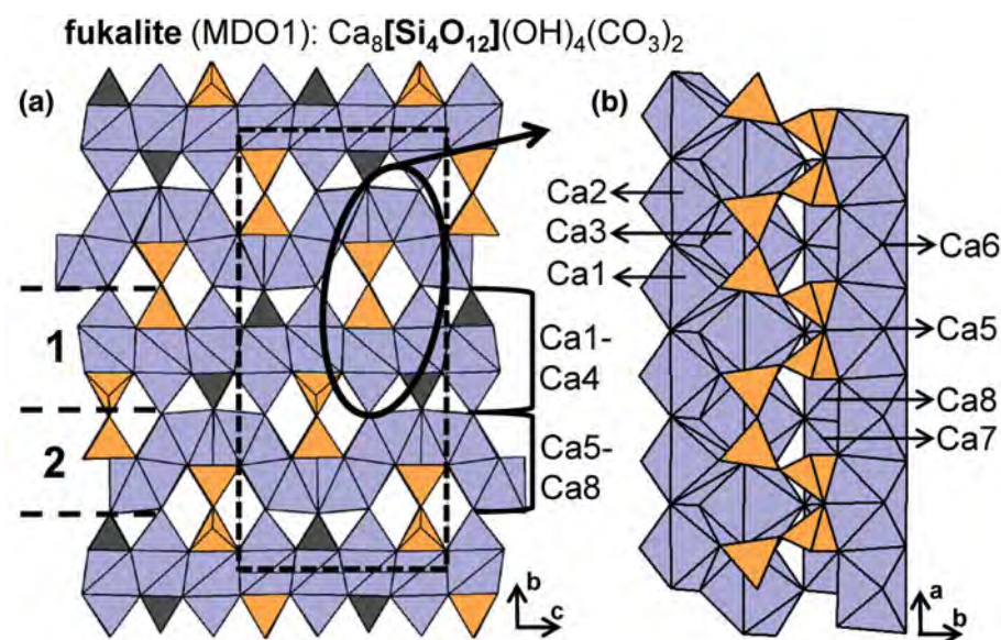
Fig. 21. The structure of fukalite projected (a) along the a -axis and (b) onto (001). In (a), (CO 3 ) groups are shown in dark grey and H atoms associated with (OH) − groups are omitted for clarity. Fine dashed black lines outline the unit cell.
