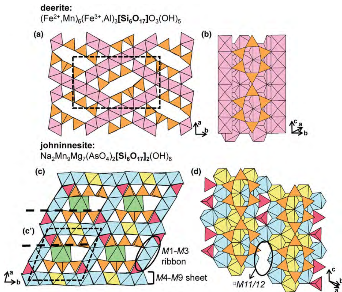
Fig. 74. The structure of deerite projected (a) along the c -axis and (b) orthogonal to the c -axis. The structure of johninnesite projected (c) along the c -axis and (d) orthogonal to the c -axis. Fine dashed black lines outline the unit cell and H atoms associated with (\text{OH})^- groups are omitted for clarity.
