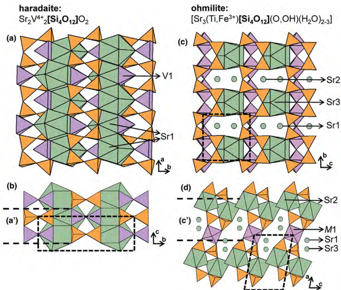
Fig. 20. The structure of haradaite projected (a) onto (001) and (b) along the a -axis (b). The structure of ohmilite projected (c) onto (100) and (d) along the b -axis (c) and into the b -axis. Fine dashed black lines outline the unit cell and H atoms associated with (OH) - and (H 2 O) groups have been omitted for clarity.
