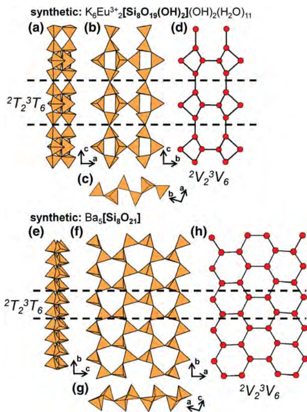
Fig. 69. (a, b, c) Tetrahedral representations of the {}^2T_2^3T_6 ribbon in synthetic K_6Eu^{3+}_2[Si_8O_{19}(OH)_2](OH)_2(H_2O)_{11} projected (a) onto (010), (b) onto (100), (c) along the c-axis and (d) a ball-and-stick (graphical) representation of the ribbon. (e, f, g) Tetrahedral representations of the {}^2T_2^3T_6 ribbon in synthetic Ba_5[Si_8O_{21}] projected (e) onto (100), (f) onto (001), (g) along the b-axis and (h) a ball-and-stick (graphical) representation of the ribbon. Dashed black lines outline the geometrical and topological repeat unit of the ribbon.
