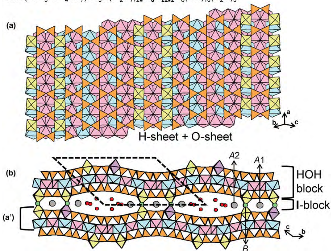
Fig. 61. The structure of veblenite highlighting the (a) H- and O-sheet projected onto (001) and the (b) HOH-block and I-block viewed along the a -axis. Here, I-block, (\text{H}_2\text{O}) groups are shown as red circles. Fine dashed black lines outline the unit cell and H atoms associated with (\text{OH})^- groups are omitted for clarity.
