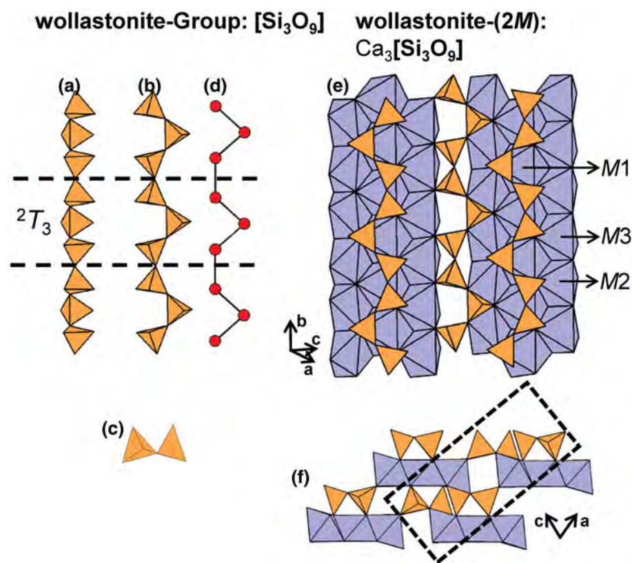
Fig. 11. (a, b, c) Tetrahedral representations of the 2T_3 chain in wollastonite-group minerals and (d) a ball-and-stick representation of the chain. The structure of wollastonite-2M viewed (e) orthogonal to the b -axis and (f) along the b -axis. Dashed black lines show the geometrical repeat unit of the chain and fine dashed black lines outline the unit cell.
