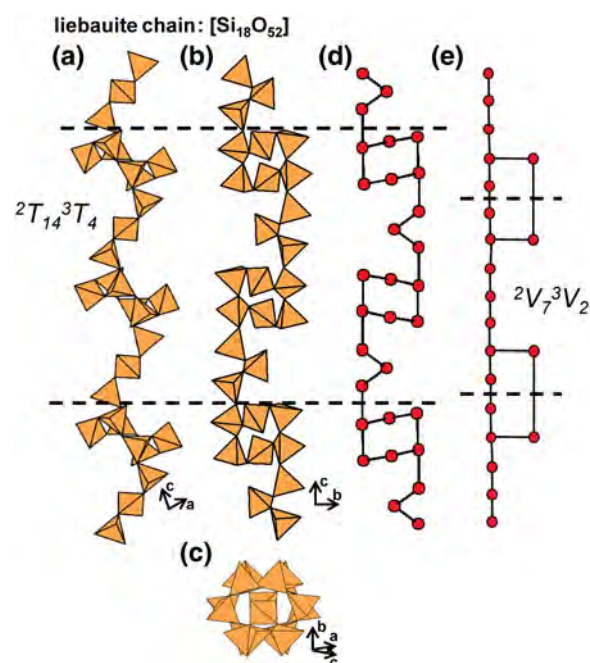
Fig. 88. (a, b, c) Tetrahedral representations of the {}^2T_{14}{}^3T_4 chain in liebauite projected (a, b) orthogonal to [10\bar{1}] , (c) along [10\bar{1}] , (d) a ball-and-stick and (e) a graphical representation of the chain. Dashed black lines outline the geometrical and topological repeat unit of the chain.
