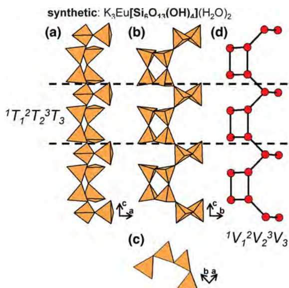
Fig. 90. (a, b, c) Tetrahedral representations of the ^1T_1\ ^2T_2\ ^3T_3 ribbon in synthetic \text{K}_3\text{Eu}[\text{Si}_6\text{O}_{13}(\text{OH})_4](\text{H}_2\text{O})_2 projected (a) onto (010), (b) onto (100), (c) along the c -axis and (d) a ball-and-stick (graphical) representation of the ribbon. Dashed black lines outline the geometrical and topological repeat unit of the ribbon.
