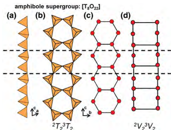
Fig. 62. (a, b) Tetrahedral representations of the {}^2T_2{}^3T_2 ribbon in amphibole supergroup minerals projected (a) orthogonal to the c -axis, (b) onto (100), (c) a ball-and-stick and (d) a graphical representation of the ribbon. Dashed black lines outline the geometrical and topological repeat unit of the ribbon.
