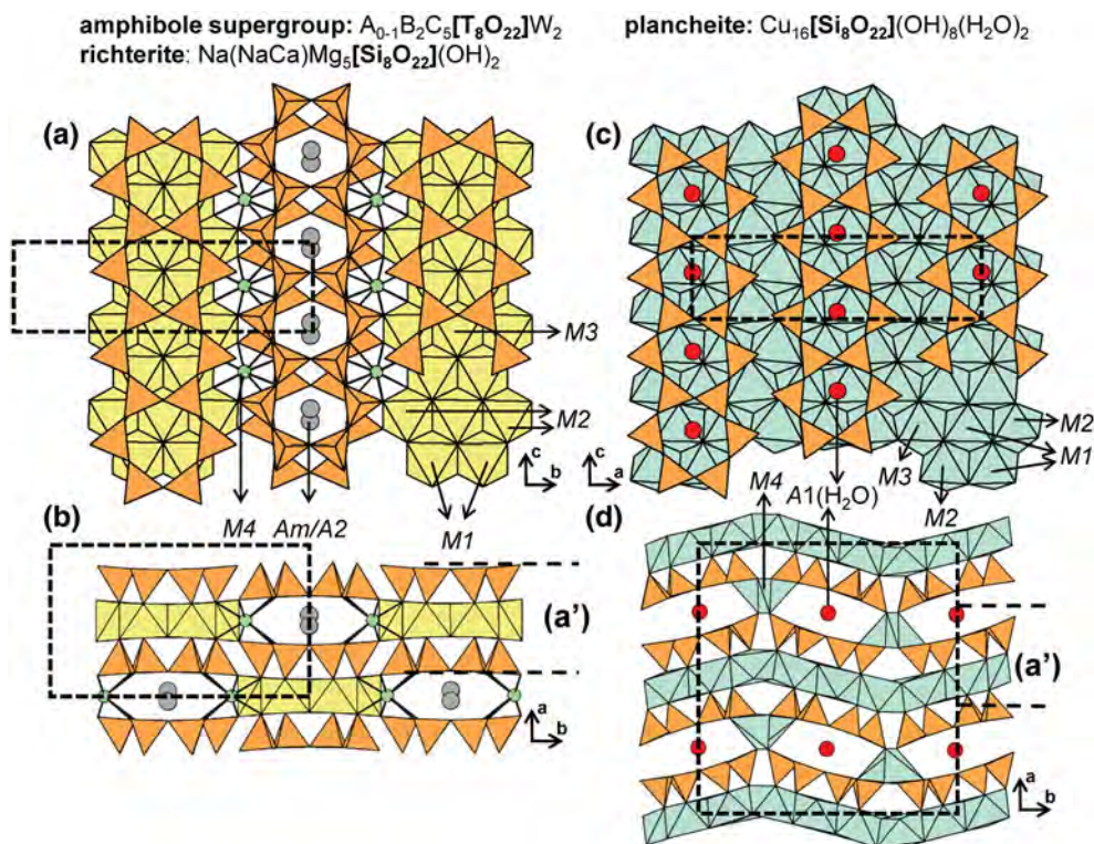
Fig. 63. The structure of richterite projected (a) onto (100) and (b) along the c -axis (a). The structure of plancheite projected (c) onto (100) and (d) along the c -axis. Fine dashed black lines outline the unit cell and H atoms associated with (OH) − groups are omitted for clarity
