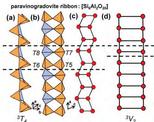
Fig. 35. (a, b) Tetrahedral representation of the ^3T_4 ribbon in paravinogradovite projected (a) orthogonal to the a -axis (b) onto (010), (c) a ball-and-stick and (d) a graphical representation of the ribbon. The T8 site is occupied by \text{Al}^{3+} . Dashed black lines outline the geometrical and topological repeat unit of the ribbon.
