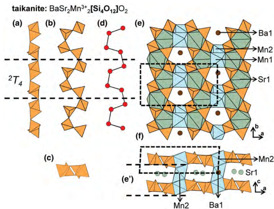
Fig. 22. (a, b, c) Tetrahedral representations of the 2 T 4 chain in taikanite and (d) a ball-and-stick representation of the chain. The structure of taikanite projected (e) onto (001) and (f) along the b -axis. Dashed black lines outline the geometrical repeat unit of the chain and fine dashed black lines outline the unit cell.
