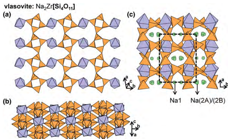
Fig. 82. The structure of vlasovite projected approximately (a) orthogonal to [101] , (b) onto [101] where \text{Na}^+ ions have been omitted and (c) along the c -axis where \text{Na}^+ ions occur in channels parallel to the c -axis. Fine dashed black lines outline the unit cell.
