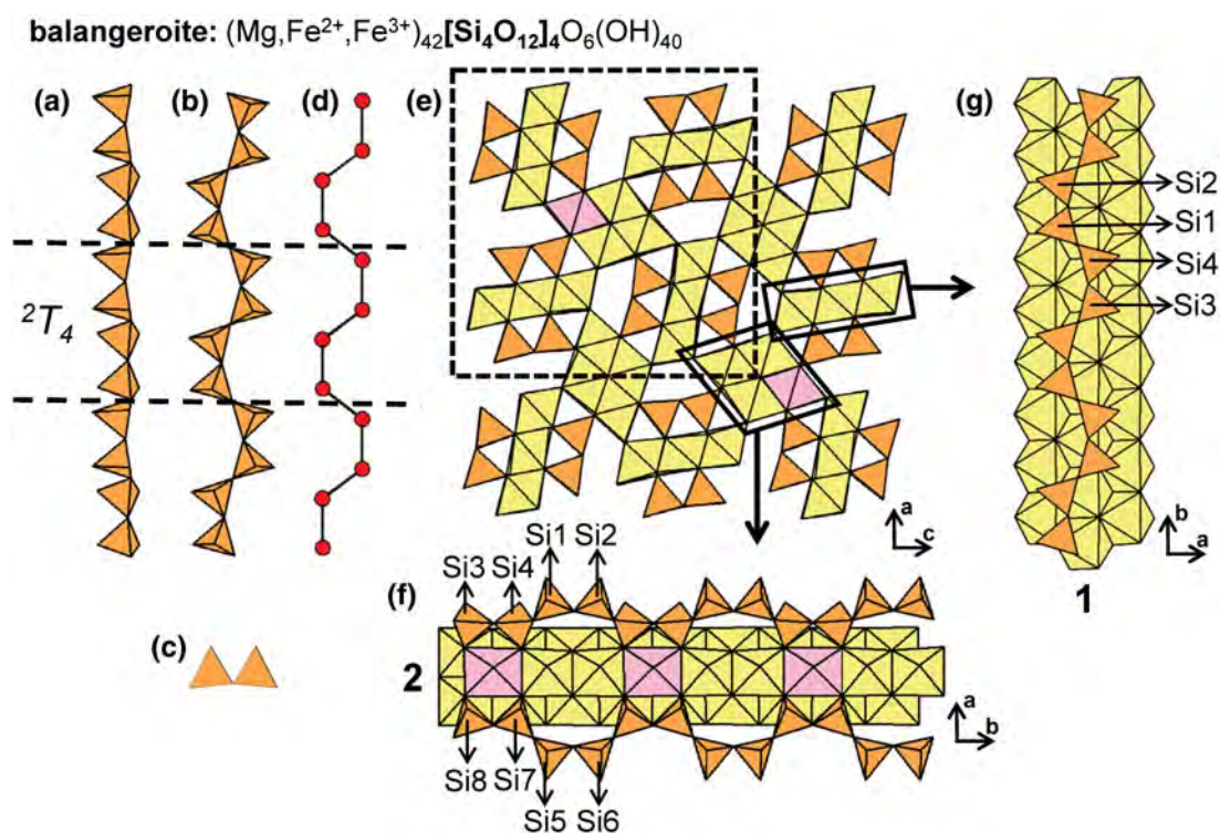
Fig. 24. (a, b, c) Tetrahedral representations of the ^2T_4 chain in balangeroite and (d) a ball-and-stick representation of the chain. The structure of balangeroite projected (e) along the b -axis and (f, g) the two modes of linkage between ^2T_4 chains and the interstitial structure projected onto (001). Dashed black lines outline the geometrical repeat unit of the chain and fine dashed black lines outline the unit cell. The H atoms associated with (\text{OH})^- groups have been omitted for clarity.
