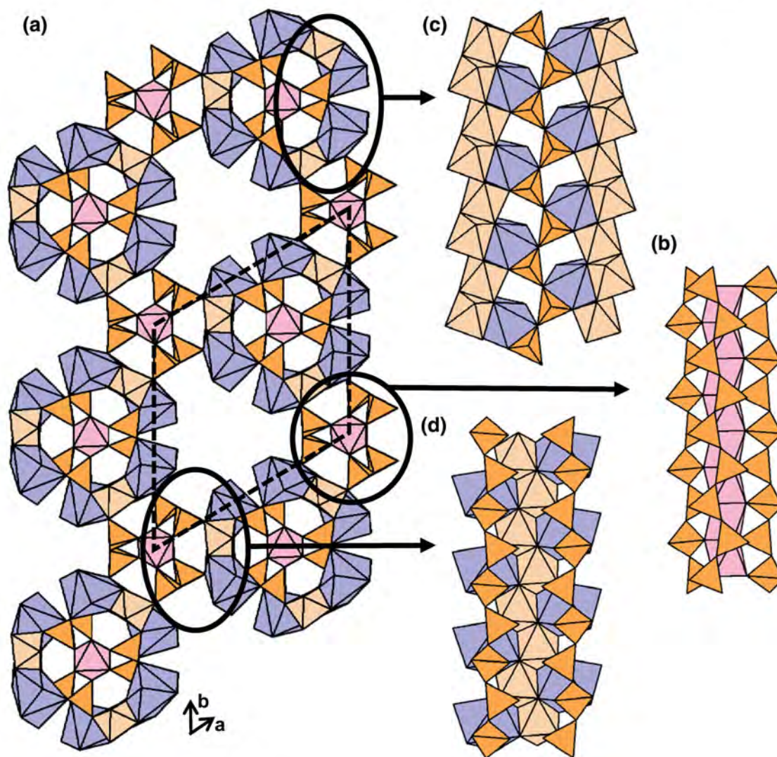
Fig. 10. The structure of aerinite projected (a) along the c -axis and (b, c, d) the structural modules that contain ^2T_2 chains viewed orthogonal to the c -axis. Fine dashed black lines outline the unit cell and H atoms associated with (\text{OH})^- and (\text{H}_2\text{O}) groups and C atoms associated with (\text{CO}_3) groups have been omitted for clarity.
