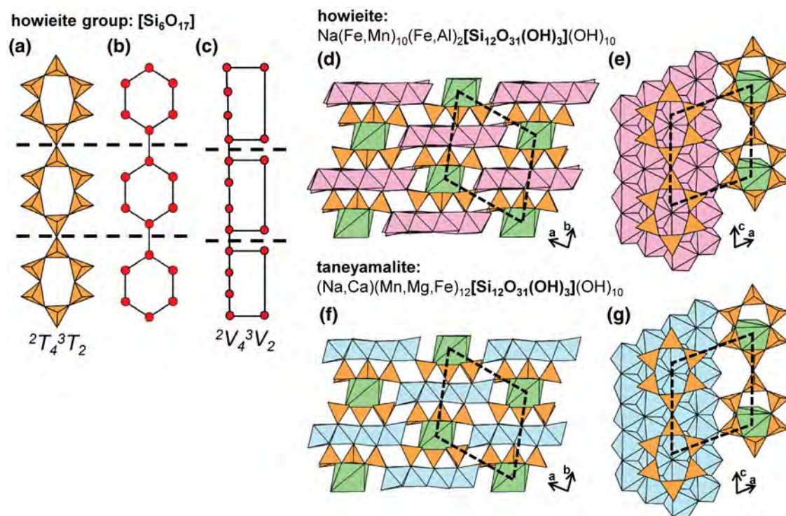
Fig. 73. (a, b, c) Tetrahedral representation of the {}^2T_4{}^3T_2 chain in howieite-group minerals, (b) a ball-and-stick and (c) a graphical representation of this chain. The structure of howieite projected (d) along the c -axis and (e) onto (010). The structure of taneyamalite projected (f) along the c -axis and (g) onto (010). Dashed black lines outline the geometrical and topological repeat unit of the ribbon and fine dashed black lines outline the unit cell. The H atoms associated with (OH) − groups are omitted for clarity
