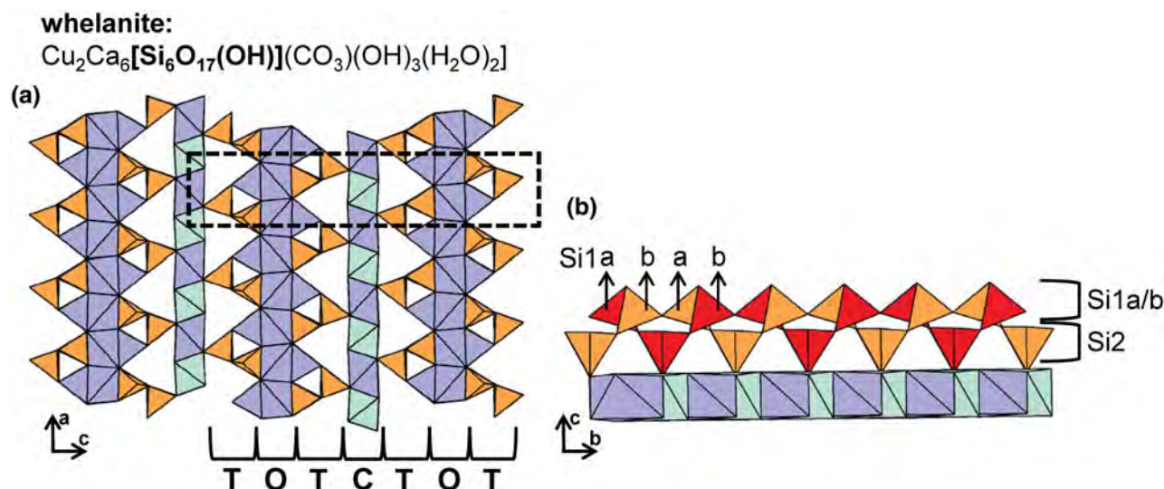
Fig. 18. The structure of whelanite projected (a) along the b -axis and (b) onto (100). In (a), the TOTCTOT stacking sequence is labelled and in (b) one of the overlapping, half-occupied ^2T_3 chains is shown as orange tetrahedra on the other chain is shown as red tetrahedra. Fine dashed black lines outline the unit cell and H atoms associated with (\text{OH})^- and (\text{H}_2\text{O}) groups and C atoms associated with (\text{CO}_3) groups have been omitted for clarity.
