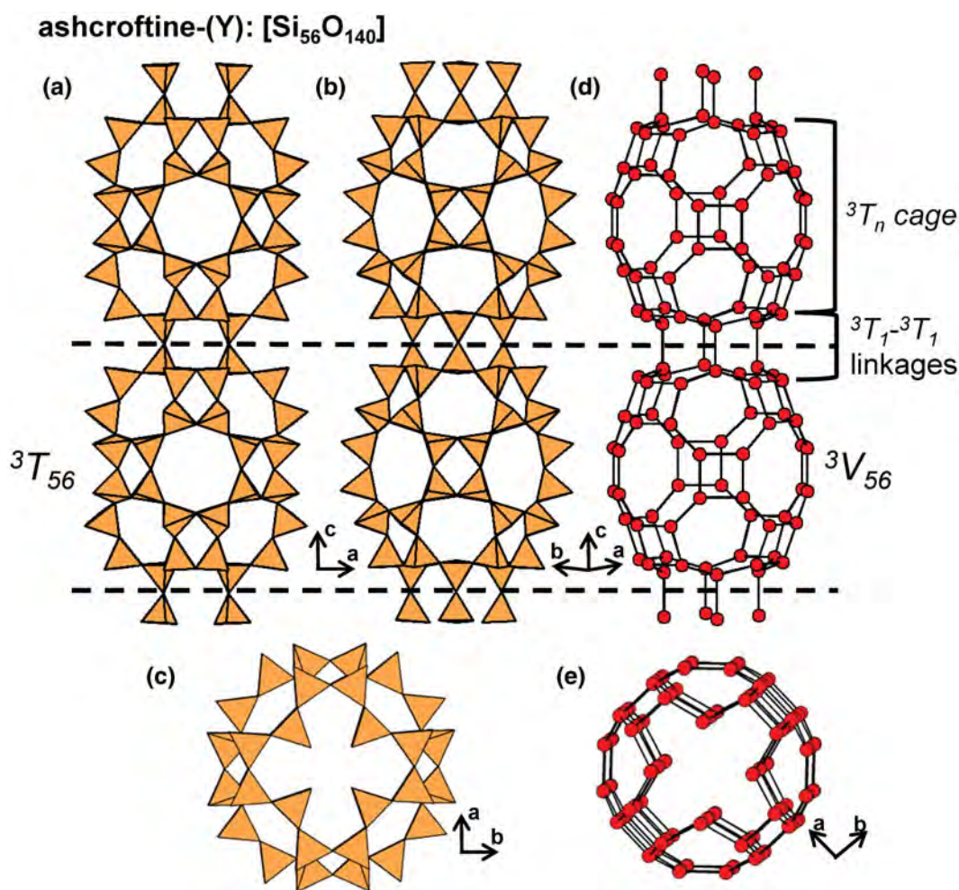
Fig. 54. (a, b, c) Tetrahedral representation of the ^3T_{56} tube in ashcroftine projected (a) onto (010), (b) orthogonal to the c-axis, (c) along the c-axis, and (d, e) a ball-and-stick (graphical) representation of the tube. Dashed black lines outline the geometrical and topological repeat unit of the tube.
