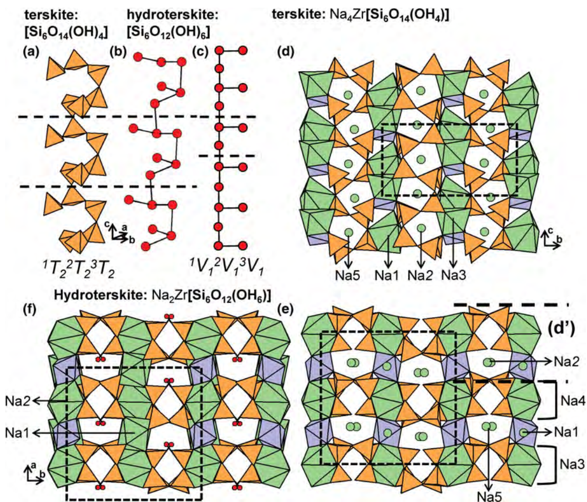
Fig. 95. (a) Tetrahedral and (b) ball-and-stick representation of the 1T_2^2T_2^3T_2 chain in terskite and hydroterskite and (c) a graphical representation of the 1V_1^2V_1^3V_1 chain. The structure of terskite projected (d) onto (100) and (e) along the c -axis where H atoms associated with (\text{OH})^- groups are omitted. The structure of hydroterskite projected (f) along the c -axis where one of three H sites associated with (OH) groups is shown which is replaced by \text{Na}^+ ions in terskite . Dashed black lines outline the geometrical and topological repeat unit of the chain and fine dashed black lines outline the unit cell.
