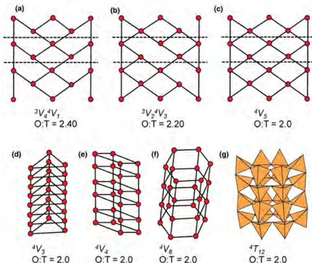
Fig. 106. The graphical representation of ribbons and tubes with O:T = 2.0 \leq x \leq 2.5 that are not observed in minerals. (a) {}^3V_4^4V_1 ( O:T = 2.40 ), (b) {}^3V_2^4V_3 ( O:T = 2.20 ), and (c) {}^4V_5 ( O:T = 2.0 ) ribbon graphs. (d) {}^4V_3 (triangles), (e) {}^4V_4 (squares), and (f) {}^4V_6 (hexagons) tube graphs where O:T = 2.0 and (g) a tetrahedral representation of a {}^4T_{12} tube that is topologically identical to the tube shown in (f). Dashed black lines outline the repeat unit of the graphs in (a), (b) and (c).
