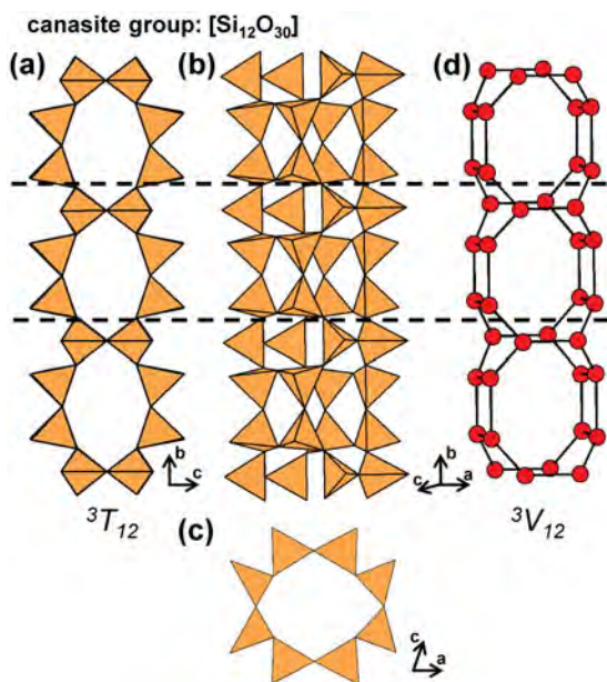
Fig. 48. (a, b, c) Tetrahedral representation of the ^3T_{12} tube in canasite projected (a) onto (100), (b) orthogonal to the b -axis, (c) along the b -axis and (d) a ball-and-stick (graphical) representation of the tube. Dashed black lines outline the geometrical and topological repeat unit of the tube.
