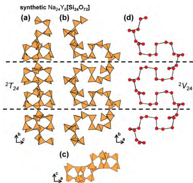
Fig. 34. (a, b, c) Tetrahedral representations of the ^2T_{24} chain in synthetic \text{Na}_{24}\text{Y}_8[\text{Si}_{24}\text{O}_{72}] projected (a) onto (100), (b) onto (001), (c) along the b -axis and (d) a ball-and-stick representation of the chain. Dashed black lines outline the geometrical repeat unit of the chain.
