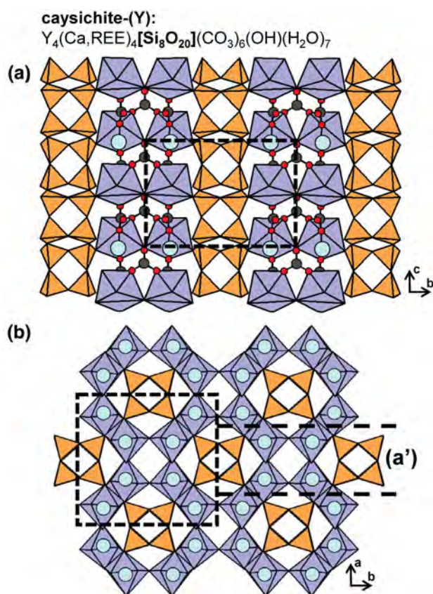
Fig. 41. The structure of caysichite-(Y) projected (a) onto (100) and (b) along the c -axis. In (a), the C and O atoms of the (CO_3) groups are shown as dark grey and red circles, respectively. In (a) and (b), Y^{3+} ions are shown as teal circles. In (a), H atoms associated with (H_2O) and (OH)^- groups are omitted and in (b) C atoms associated with (CO_3) groups are also omitted for clarity. Fine dashed black lines outline the unit cell.
