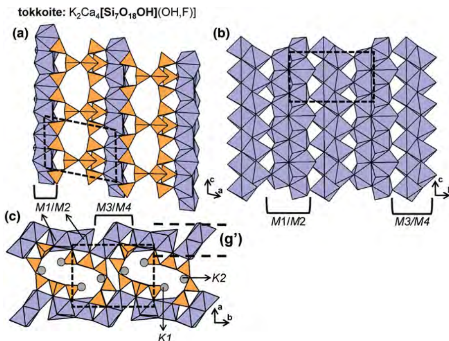
Fig. 72. The structure of tokkoite projected (a) onto (010) showing the linkage of 2T_3^3T_4 ribbons to sheets of \text{Ca}^{2+} -polyhedra, (b) sheets of \text{Ca}^{2+} -polyhedra projected onto (100) and (c) the alternating layers of 2T_3^3T_4 ribbons and sheets of \text{Ca}^{2+} -polyhedra projected along the c -axis. Fine dashed black lines outline the unit cell and H atoms associated with (OH) − groups are omitted for clarity.
