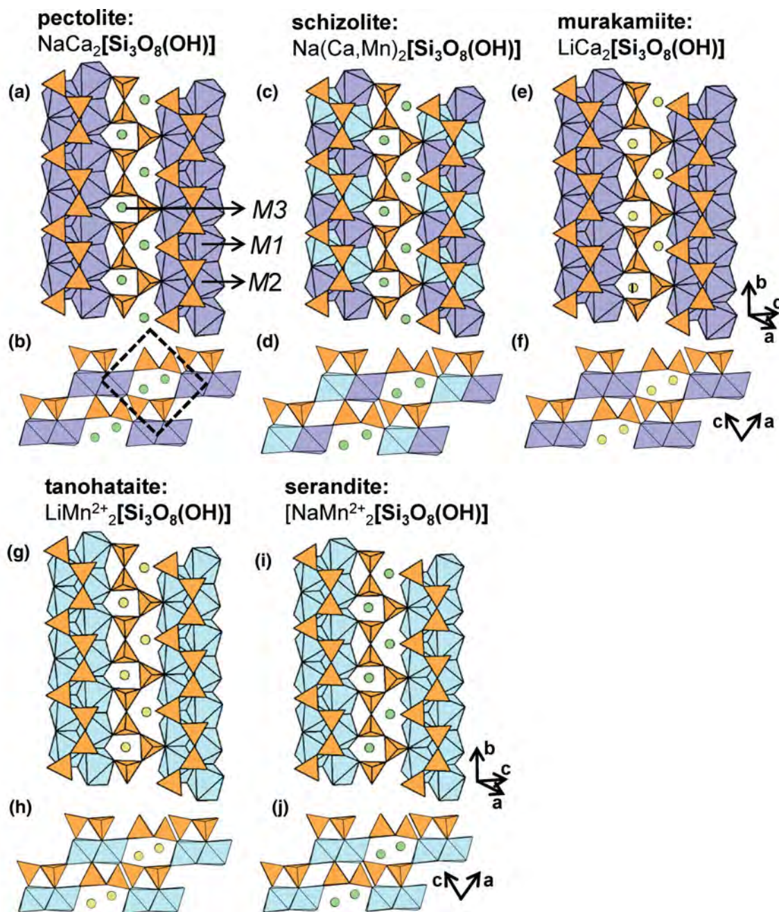
Fig. 13. The structure of (a, b) pectolite , (c, d) schizolite , (e, f) murakamiite , (g, h) tanohataite and (i, j) serandite viewed (a, c, e, g, i) orthogonal to the b -axis and (b, d, f, h, j) along the b -axis. M -site labels in (a) are also applicable to (c), (e), (g) and (i) and fine dashed black lines outline the unit cell. The H atoms associated with (OH) − groups have been omitted for clarity.
