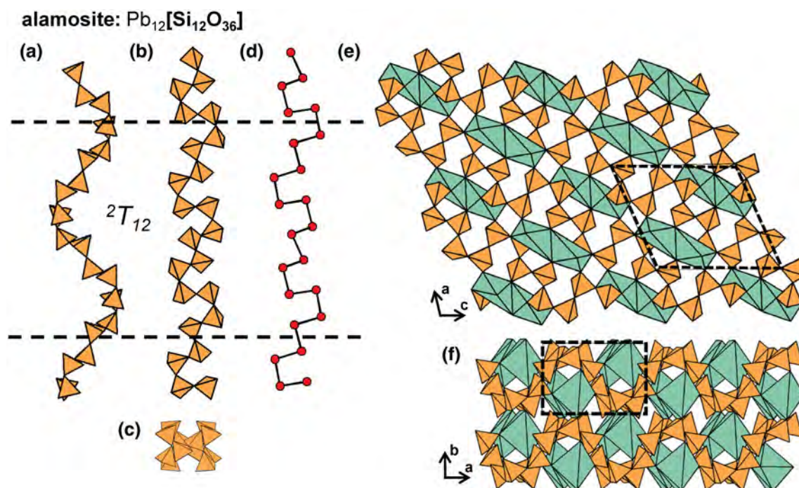
Fig. 33. (a, b, c) Tetrahedral representations of the ^2T_{12} chain in alamosite and (d) a ball-and-stick representation of the chain. The structure of alamosite projected (e) onto (010) and (f) along the c -axis. Pb1 and Pb2 atoms have been omitted for clarity. Dashed black lines outline the geometrical repeat unit of the chain and fine dashed black lines outline the unit cell.
