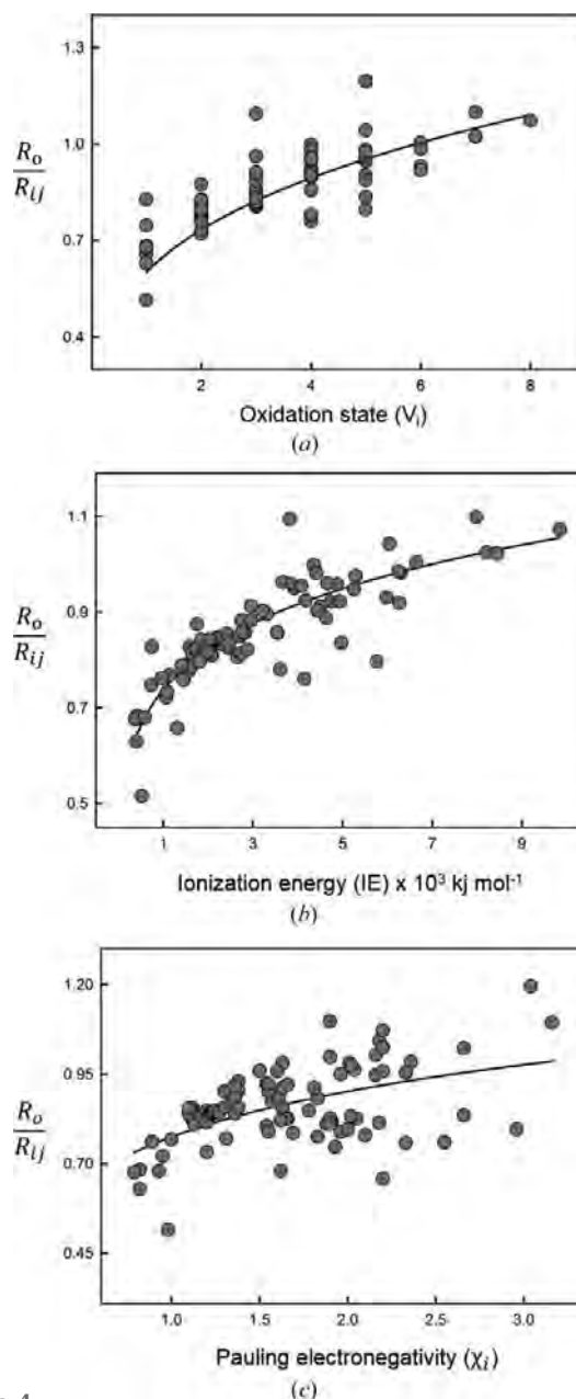
Figure 4 Relation between bond-valence parameter R_o divided by mean bond length and (a) oxidation state, (b) ionization energy and (c) Pauling electronegativity.
