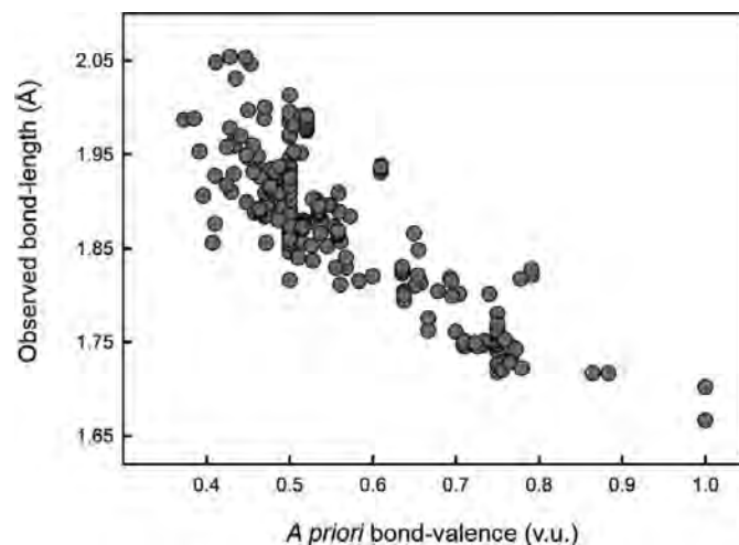
Figure 2 Determination of the curvature of the bond-valence relation by a match of the a priori bond valences to their observed bond lengths.
