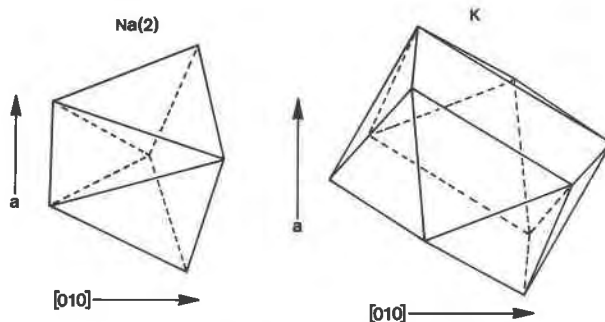
Fig. 1. Selected coordination polyhedra in ungemachite: left—the Na(2) 6 distorted trigonal prism; right—the K 10 polyhedron.
