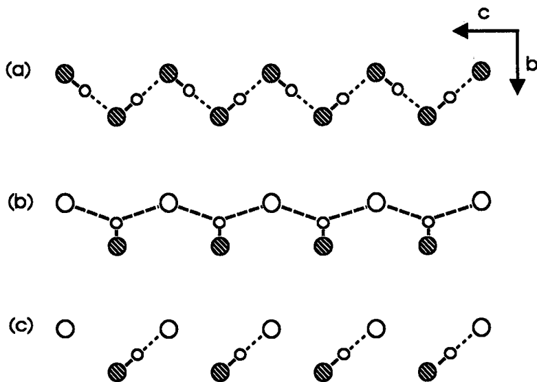
FIG. 7. Possible local F-OH arrangements along the hydrogen-bonded strips in hambergite. (a) All sites are occupied by OH, (b) one half the sites are occupied by F, the \text{OH}(4)f\text{-H} bond is parallel to the b direction, and the H atom forms a bifurcated hydrogen bond with adjacent F atoms; (c) one half the sites are occupied by F with the occurrence of hydrogen-bonded OH-F pairs. O atoms are shown as circles shaded with parallel lines, F atoms are large open circles, and H atoms are shown as small open circles.
