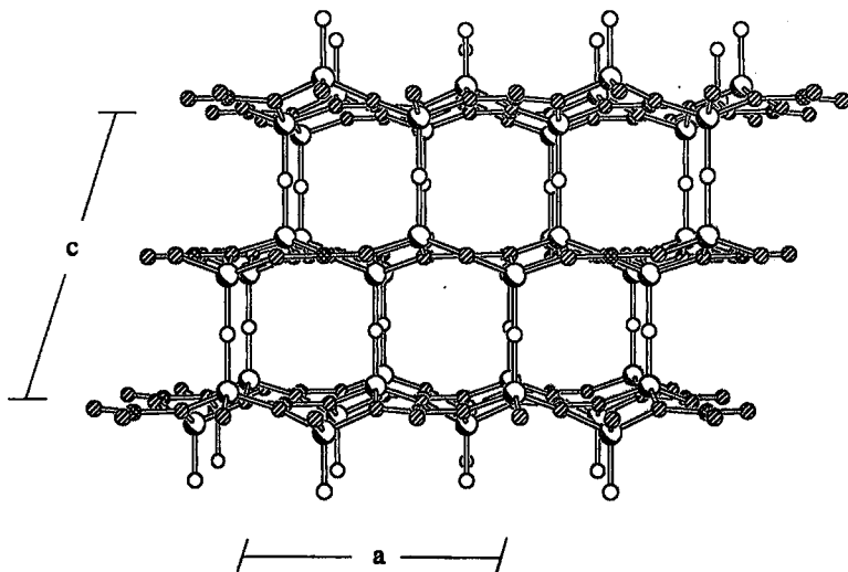
FIG. 5. The structure of Be_2(BO_3)F projected down [010]. B atoms are shown as cross-hatched circles, Be atoms as open circles with shading in the lower left, O atoms as circles shaded with parallel lines, and F atoms are shown as open circles.
