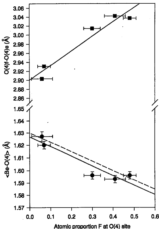
FIG. 4. The effect of F \leftrightarrow OH substitution upon the \langle Be-O(4) \rangle and O(4)f-O(4)e separations. The best fit line for \langle Be-O(4) \rangle versus F is \langle Be-O(4) \rangle = -0.077F + 1.627 , r = 0.934 , and for O(4)f-O(4)e versus F , it is O(4)f-O(4)e = 0.322F + 2.900 , r = 0.968 . The broken line represents the expected variation of \langle Be-O(4) \rangle obtained from sums of ionic radii.
