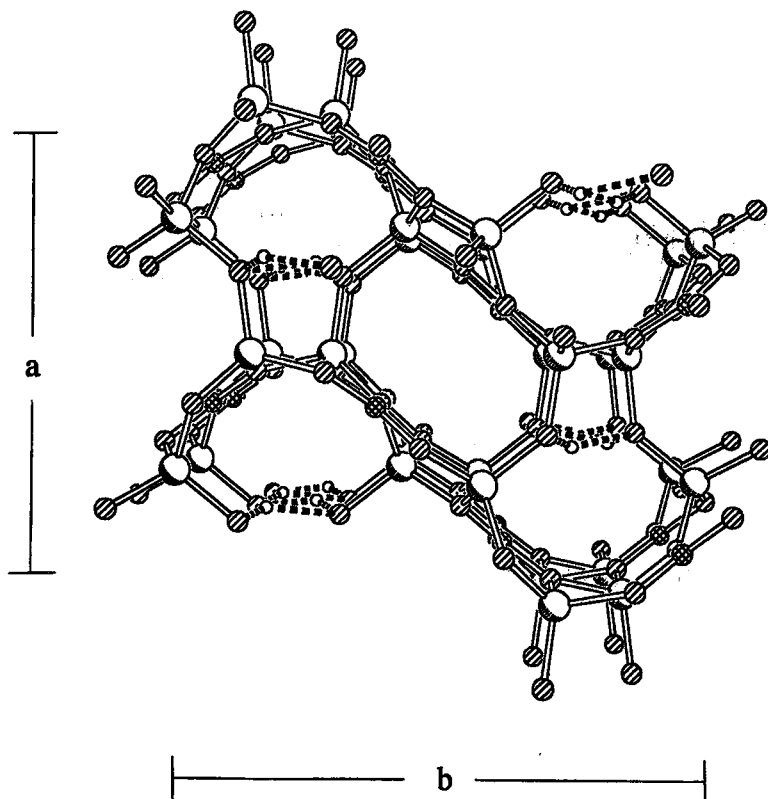
FIG. 1. The structure of hambergite projected down [001]. B atoms are shown as cross-hatched circles, Be atoms as open circles with shading in the lower left, O atoms as circles shaded with parallel lines, H atoms are shown as small open circles. Hydrogen bonds are shown as broken heavy lines.
