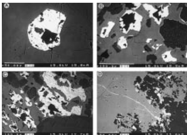
FIGURE 1. BSE images of rubicline from Elba: (A) Large grain of rubicline (white) + quartz (black) in microcline (dark gray); (B) Rubicline (white) including grains of quartz (black) in microcline (gray) associated with albite (black) and muscovite (mottled dark gray); (C) Rubicline (white) + quartz (black) in microcline (gray) in contact with Rb-free adularia (dark gray) at margins; (D) Veinlet of rubicline (white) in microcline (gray) and small grains of rubicline (white) associated with albite (black).
