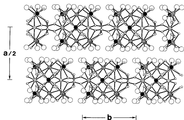
FIGURE 8. The crystal structure of georgeericksenite projected along [001]; legend as in Figures 6 and 7.
