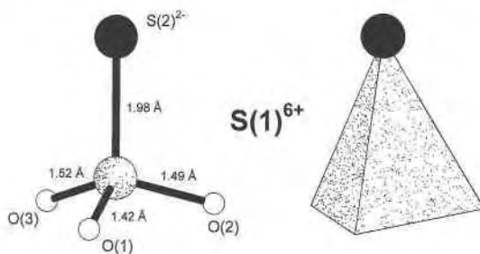
FIG. 2. The coordination of the S (1) site, shown as atoms (left) and as a tetrahedron (right) in which the S (2) atom is identified as a large black circle; legend as in Figure 1, with a large random-dot-shaded circle as the S (1) site.
