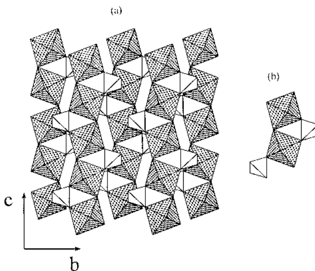
FIGURE 2. The kieselite structure type. (a) The framework with the characteristic 7 Å octahedral chains. (b) The FBB of the kieselite structure type.
