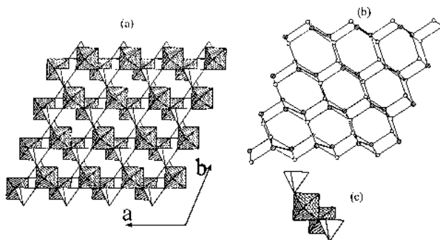
FIGURE 1. The structure of schubnelite. (a) Projected onto (001), showing one double layer of edge-sharing octahedra and isolated (\text{VO}_4) tetrahedra. (b) The schubnelite framework with a two-dimensional 6^3 net parallel to (001) and 4^4 nets parallel to (100) and (010). The shared octahedral edge is shown as a bold line between octahedral nodes. (c) The FBB of the schubnelite structure.
