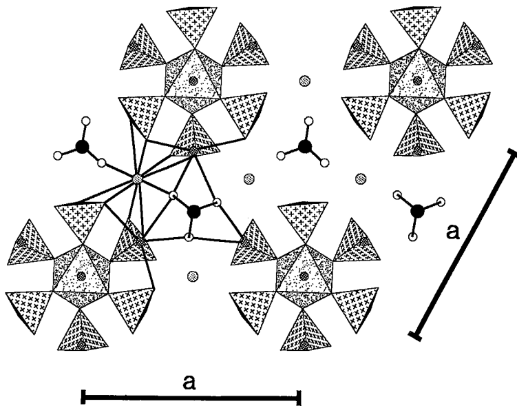
FIG. 2. The structure of humberstonite viewed down [001]. ( \text{MgO}_6 ) octahedra are shaded with a random dot pattern, ( \text{SO}_4 ) tetrahedra are shaded with crosses, Na atoms are cross-hatched circles, K atoms are dotted circles, N and O atoms are solid and open circles, respectively. N-O and selected Na-O and K-O bonds are given as solid lines.
