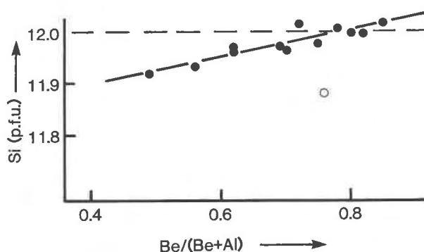
Fig. 7. Variation in Si (apfu) as a function of Be/(Be + Al) in milarites; the chemical data are taken from Černý et al. (1980). The open circle is the analysis of Tittling milarite (no. 33 of Černý et al., 1980); the analysis of this milarite sample given in Table 1 shows that this sample does lie on the observed trend.
