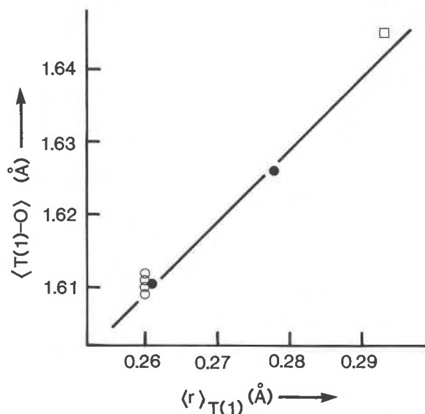
Fig. 11. Variation in \langle T1-O \rangle with constituent cation radius at the T1 site for the milarite-group minerals; the filled circles are the mean values of the data for milarites and osumilite, and the line is drawn through these two points; other data are marked by hollow symbols, except the open square = armenite.
