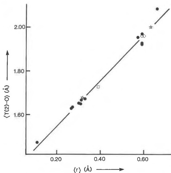
Fig. 12. Variation in \langle T2-O \rangle as a function of constituent cation radius at the T2 site for the milarite-group minerals; filled circles are data points that we consider more reliable, and the stars indicate data for the related structures of lithium cesium beryl (Hawthorne and Černý, 1977) and tuhualite (Merlino, 1969); data for zektzerite (Ghose and Wan, 1978) also lies on the line; open circle = sogdianite, open square = armenite, open diamond = zinc milarite.
