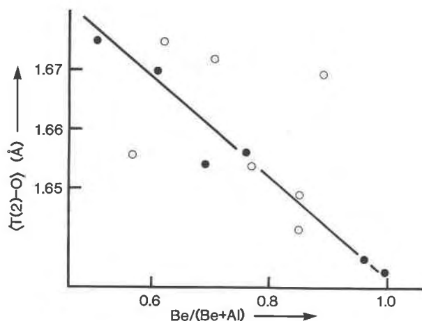
Fig. 8. Variation in \langle T2-O \rangle as a function of Be/(Be + Al) in milarites; filled symbols indicate site occupancies derived from unconstrained site-occupancy refinement, and hollow symbols denote occupancies derived from the chemical analyses.
