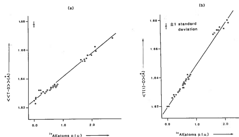
Fig. 3. — a) Variation in grand \langle T-O \rangle distance with total ^{IV}Al (tetrahedrally coordinated aluminium) in the C2/m amphiboles for which external chemical analyses are available (■); □ denote values derived from a slightly different equation by Ungaretti et al. (1981b) and Ungaretti et al. (1983). b) variation in \langle T(1)-O \rangle distance with total ^{IV}Al in the C2/m amphiboles; legend as for (a).
