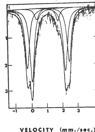
Fig. 10. – The Mössbauer spectrum of synthetic 'ferro-actinolite' ("ferrotremolite"); from Burns and Greaves (1971).
