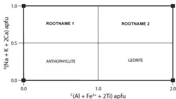
FIGURE 1. Orthorhombic magnesium-iron-manganese amphiboles and their compositional boundaries. Filled black squares are the locations of named and unnamed Mg end-members.
