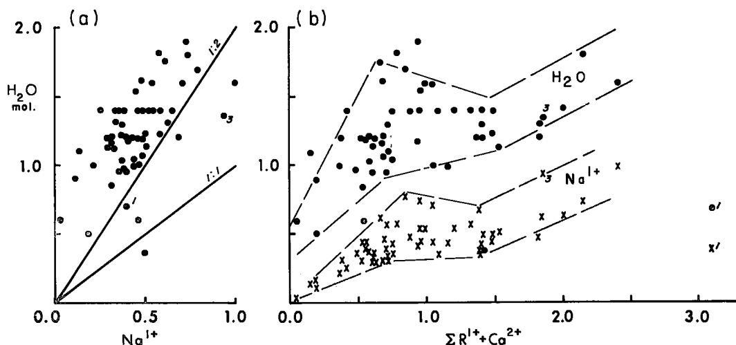
FIG. 2. \text{H}_2\text{O} content of beryl (mol. %) compared to the \text{Na}^+ content (a) and to the \Sigma \text{R}^+ + \text{Ca} content (b). Data from Sosiedko (1957) 3 samples with the richest in alkalis marked 3; Deer et al. (1962), 8 samples; Vorma et al. (1965), 9 samples; Evans & Mrose (1966), 1 sample marked 1; Gordiyenko (1970), 5 samples; Bakakin et al. (1970), 22 samples; Hall & Walsh (1971), 6 samples; and Černý & Simpson (in prep.), 3 samples. Note that in (a) most beryls contain \text{H}_2\text{O} in excess of the 1:2 ratio, and that the general shape of the main \text{H}_2\text{O} field (dots) in (b) corresponds to that of \text{Na}^+ (X).
