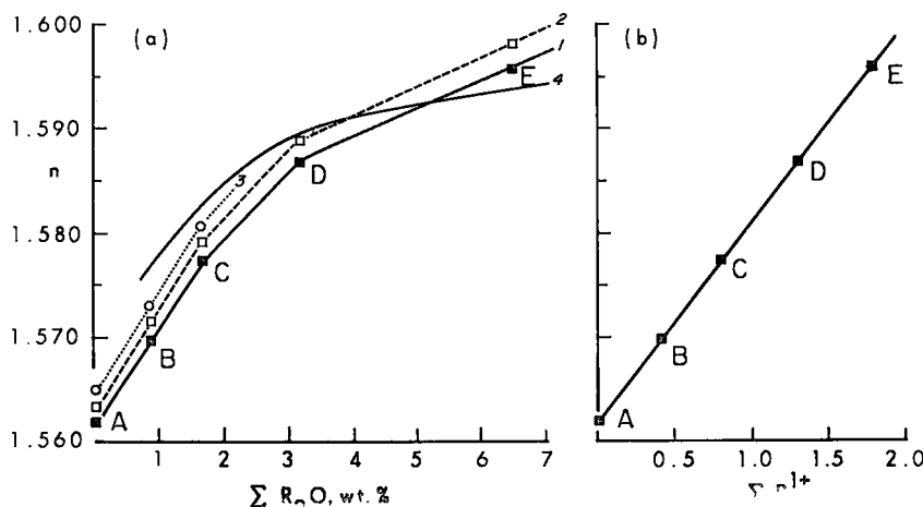
FIG. 4. Calculated n_m of simplified beryl compositions vs. \Sigma R_2O in wt. % (a) and vs. \Sigma R^+ in atomic contents (b). In (a), calculated n_m values from Table 1 (line 1, solid squares), adjusted to probable n_o using n_m = (2n_o + n_e)/3 (line 2, empty squares), and corrected for about 0.5 wt. % Fe_2O_3 (line 3, empty circles), are compared to the same relationship in natural beryls (line 4, redrawn from Fig. 3); see text for comments. In (b), calculated n_m shows almost the same rate of increase with Cs^+ (points D to E) as with Na^+ + 2H_2O (points A to C).
