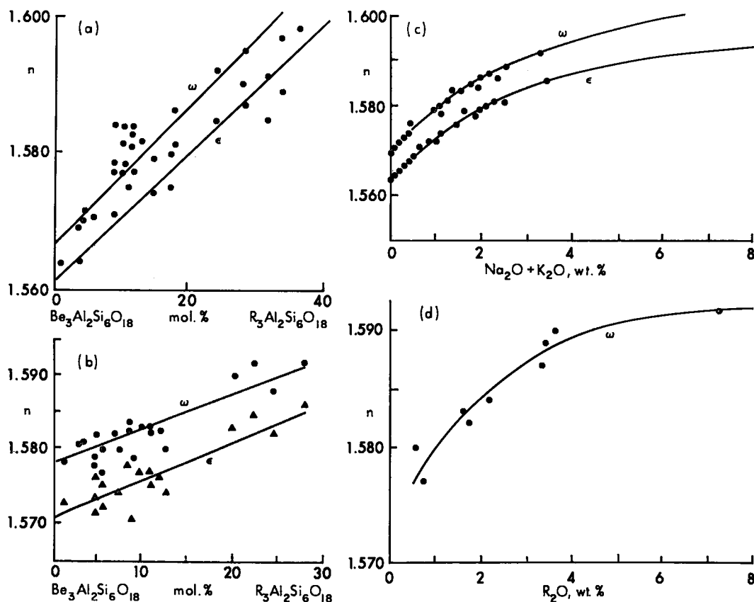
FIG. 1. Correlation of alkali contents with refractive indices of beryl by (a) Winchell (1951), (b) Deer et al. (1962), (c) Dorfman (1951), and (d) Feklitchev (1964). Plots of n_e and n_o are not distinguished in Winchell's (1951) original graph. Note the inconsistencies in the extrapolated values for \text{Be}_3\text{Al}_2\text{Si}_6\text{O}_{18} , in the slopes of the regression lines, and in the changes of birefringence with increasing " \text{R}_3\text{Al}_2\text{Si}_6\text{O}_{18} " between (a) and (b).
