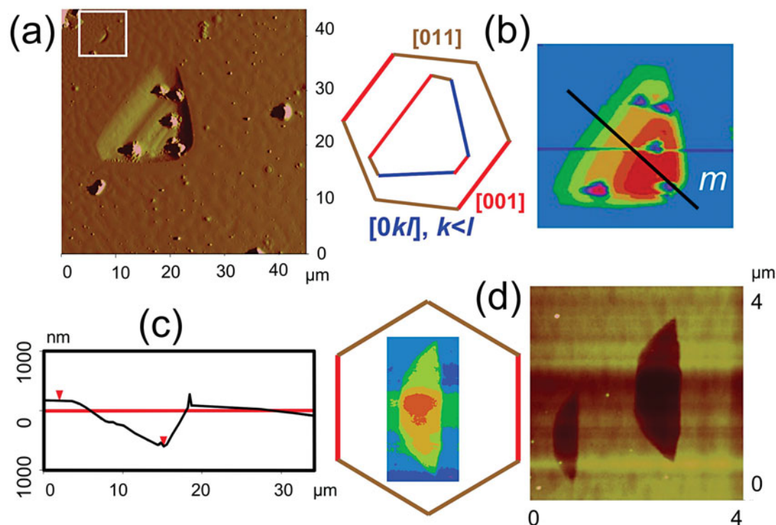
FIG. 7. (a) AFM image in deflection mode, of an etch pit formed in a \text{SrCl}_2\text{--HCl} solution of pH 2.7. (b) The orientation of the etch pit in relation to crystal morphology, and the morphology of the pit at different depths. (c) The cross section perpendicular to [001] . (d) AFM image in height mode showing the morphology and orientation of small elongate etch-pits framed in a white square box in (a).
