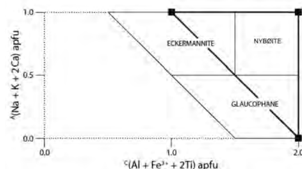
FIGURE 5. Sodium amphiboles and their compositional boundaries. The heavy solid black line is a two-dimensional section of amphibole composition space (Appendix Fig. 3) at ^{\text{B}}\text{Ca}/^{\text{B}}(\text{Ca} + \text{Na}) = 0.0 that contains sodium end-member compositions. The thick solid lines show the possible range of amphibole compositions at ^{\text{B}}\text{Ca}/^{\text{B}}(\text{Ca} + \text{Na}) = 0.0 and the solid lines to the left of the diagonal heavy solid black line show the possible range of amphibole compositions at ^{\text{B}}\text{Ca}/^{\text{B}}(\text{Ca} + \text{Na}) = 0.25 , the boundary between the sodium amphiboles and the sodium-calcium amphiboles.
