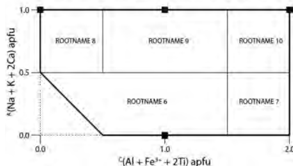
FIGURE 7. Sodium-(magnesium-iron-manganese) amphiboles and their compositional boundaries. Filled black squares are the locations of presently unnamed end-member compositions. The thick solid line refers to end-member compositions at ^B\text{Na}/^B(\text{Na} + \Sigma\text{M}^{2+}) = 0.5 . The solid lines to the left of the diagonal thick solid line show the possible range of amphibole compositions at ^B\text{Na}/^B(\text{Na} + \Sigma\text{M}^{2+}) = 0.25 , the boundary between the sodium-(magnesium-iron-manganese) amphiboles and the magnesium-iron-manganese amphiboles.
