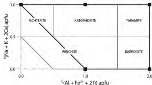
FIGURE 4. Sodium-calcium amphiboles and their compositional boundaries. The heavy solid black line is a two-dimensional section of amphibole composition space (see Appendix Fig. 3) at ^{\text{B}}\text{Ca}/^{\text{B}}(\text{Ca} + \text{Na}) = 0.5 that contains the sodium-calcium end-member compositions. The thick solid lines show the possible range of amphibole compositions at ^{\text{B}}\text{Ca}/^{\text{B}}(\text{Ca} + \text{Na}) = 0.5 and the solid lines to the left of the diagonal heavy solid black line show the possible range of amphibole compositions at ^{\text{B}}\text{Ca}/^{\text{B}}(\text{Ca} + \text{Na}) = 0.75 , the boundary between the sodium-calcium amphiboles and the calcium amphiboles.
