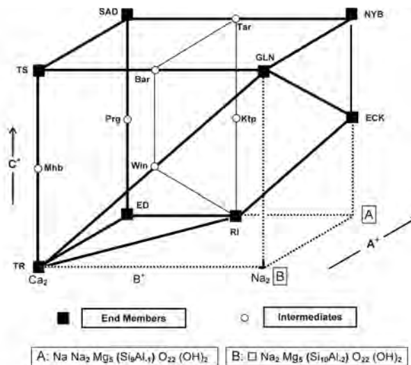
APPENDIX FIGURE 3. Compositional space for monoclinic Na-Ca-Mg-Al-Si amphiboles using {}^B\text{Na} , {}^A\text{Na} and {}^C\text{Al} as proxies for the aggregate charges of the B, A and C groups of cations. The heavy solid black lines indicate the limits of possible amphibole compositions. Filled black squares are the locations of end-members at the corners of the compositional space; open circles are the locations of end-members on the edges of compositional space. Bar = barroisite; Eck = eckermannite; Ed = edenite; Gln = glaucophane; Mhb = magnesio-hornblende; Ktp = katophorite; Nyb = nybøite; Prg = pargasite; Ri = richterite; Sad = sadanagaite; Tar = taramite; Tr = tremolite; Ts = tschermakite; Win = winchite. We use the symbols of Kretz (1983) for the amphiboles, and introduce new symbols for amphiboles not included in the original list of symbols. The full list of symbols used here for amphiboles is given as Appendix VII.
