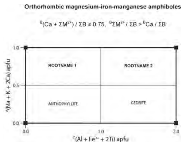
FIGURE 1. Orthorhombic magnesium-iron-manganese amphiboles and their compositional boundaries. Filled black squares are the locations of named and unnamed Mg end-members.
