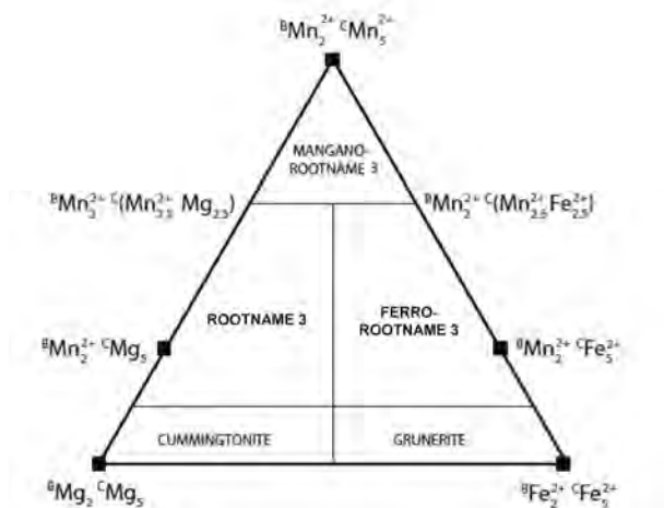
FIGURE 2. Monoclinic magnesium-iron-manganese amphiboles and their compositional boundaries. Filled black squares are the locations of named and unnamed Mg-Fe 2+ -Mn end-member compositions.
