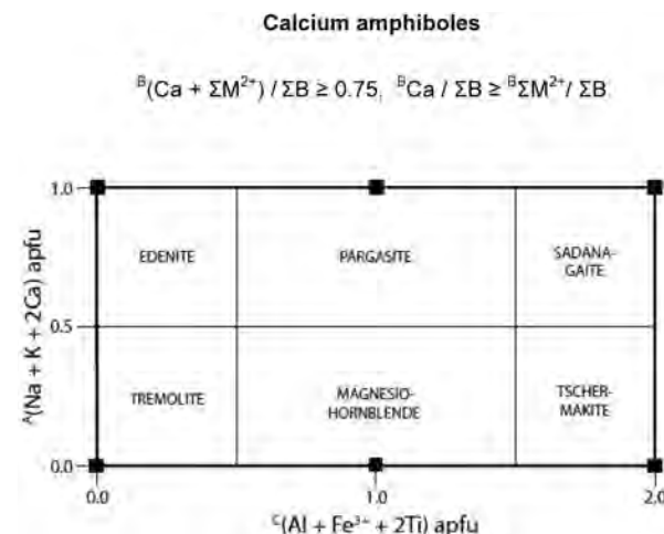
FIGURE 3. Calcium amphiboles and their compositional boundaries. The heavy solid black line is a two-dimensional section of amphibole compositional space (see Appendix Fig. 3) at ^B\text{Ca} / ^B(\text{Ca} + \text{Na}) = 1.0 that contains the calcium end-member compositions.
