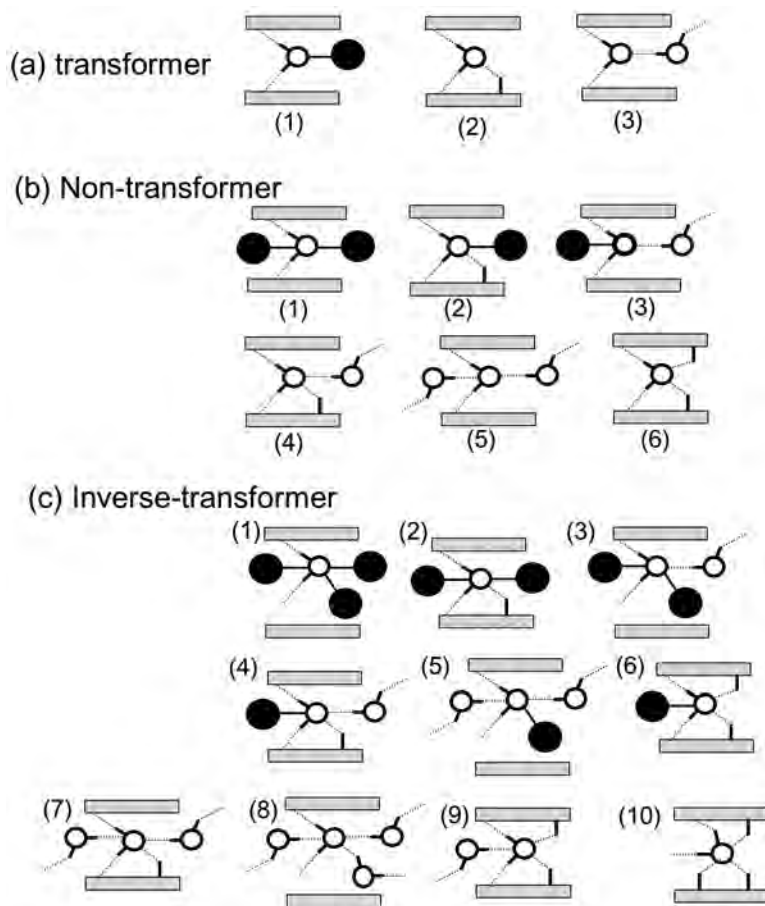
FIG. 5. Possible coordinations of (\text{H}_2\text{O}) groups (circle) by cations (black circle), other (\text{H}_2\text{O}) groups or (\text{OH}) groups of the structural unit (grey rectangle; hydrogen bonds are dashed lines); (a) transformer (\text{H}_2\text{O}) , ^{13}\text{O} ; (b) non-transformer (\text{H}_2\text{O}) groups, ^{14}\text{O} ; (c) inverse-transformer (\text{H}_2\text{O}) groups, ^{15}\text{O} .
