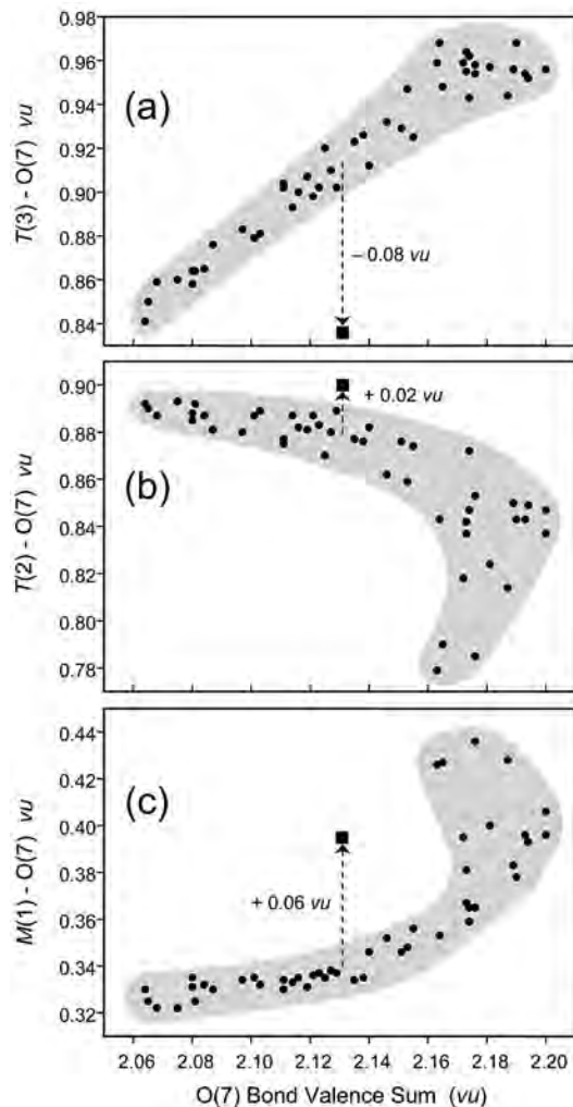
FIG. 5. Variation in individual bond-valences at the O(7) anion for the kornepurine structures of Cooper et al. (2009a). Data points are shown in black, and the fields of data are shaded grey for emphasis; data for K53 are shown as squares, and their displacement from the center of each field is marked by a broken arrow.
