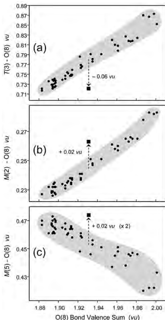
FIG. 6. Variation in individual bond-valences at the O(8) anion for the kornerupine structures of Cooper et al. (2009a). Data points are shown in black, and the fields of data are shaded grey for emphasis; data for K53 are shown as squares, and their displacement from the center of each field is marked by a broken arrow.
