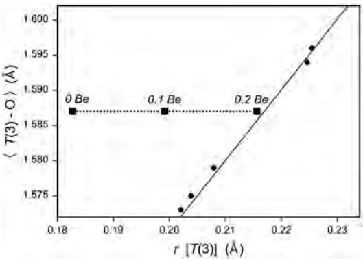
FIG. 3. The variation in <T(3)–O> as a function of constituent-cation radius for the data and regression line of Cooper et al. (2009a); only a small part of the overall variation is shown here ( cf. Fig. 1c). The black squares are the relevant refined values for K53 assuming 0.0, 0.1 and 0.2 Be apfu at T(3), respectively.
