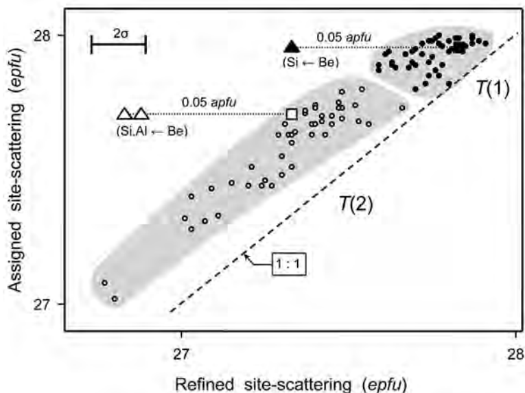
FIG. 2. The variation in assigned site-scattering as a function of refined site-scattering at the T(1) and T(2) sites for the data of Cooper et al. (2009a). Black circles: T(1) site, white circles: T(2) site; square: K53. Triangles mark hypothetical site-scattering for K53 assuming substitution of 0.05 apfu Be for Si at T(1) and for (Si,Al) at T(2) . The dashed line marks the 1:1 reference line.
