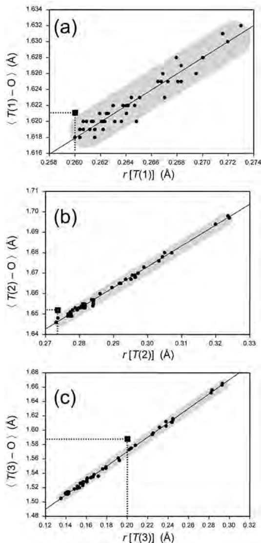
FIG. A1. The variation in \langle T-O \rangle distances as a function of constituent-cation radius for the data of Cooper et al. (2009a) (black circles) and for K53 (Table A1) (squares); also shown are the regression lines of Cooper et al. (2009a). The shaded fields denote the possible range of data that would agree with the regression lines.
