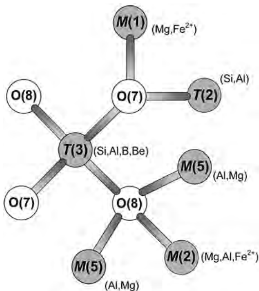
FIG. 4. Schematic view of part of the kornerupine structure around the O(7) and O(8) anions; cations are shown as grey circles, anions are shown as white circles.
