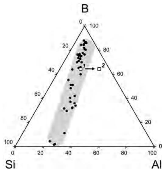
FIG. A2. The variation in Si, Al and B at the T(3) site in the kornerupine structures of Cooper et al. (2009a); legend as in Figure A1. For K53, data point 1 represents the initial T -site assignment, and data point (2) represents the readjusted T -site assignments shown in Table A1.
