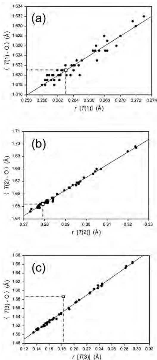
FIG. 1. The variation in \langle T-O \rangle distances as a function of constituent-cation radius for the data of Cooper et al. (2009a) (black circles) and for K53 (white square); also shown are the regression lines of Cooper et al. (2009a); the dotted lines emphasize the position of the data points for K53; (a) the T(1) site; (b) the T(2) site; (c) the T(3) site. Note that in (a) and (b), the points for K53 are constrained to lie on the regression lines, with the result that the point for K53 in (c) is significantly displaced from the regression line.
