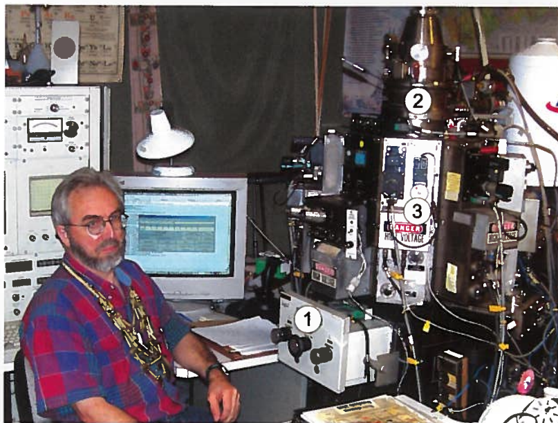
Fig.P15 Example of an Electron Microprobe. University of New Orleans, USA (A.U. Falster).
