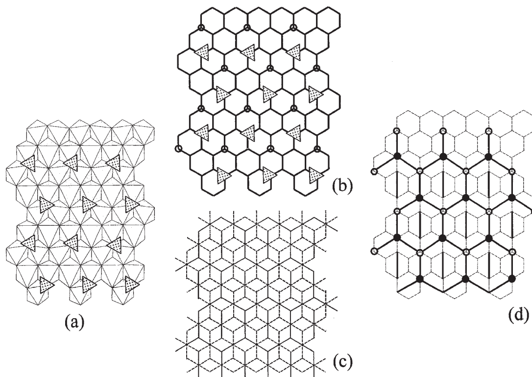
FIG. 2. (a) The decorated [\text{Cu}^{2+}\phi_2]_4 sheet in langite, [\text{Cu}^{2+}_4 (\text{SO}_4)(\text{OH})_6 (\text{H}_2\text{O})] (\text{H}_2\text{O}) , with (\text{SO}_4) and (\text{H}_2\text{O}) groups linked to the [\text{Cu}^{2+}\phi_2]_4 sheet; (b) the 6^3 net representing the shared octahedron edges of the langite [\text{Cu}^{2+}\phi_2]_4 sheet embedded into two dimensions. The decorating (\text{SO}_4) and (\text{H}_2\text{O}) (hollow circles) groups link to three-valent vertices above and below the [\text{Cu}^{2+}\phi_2]_4 sheet, respectively; (c) the 3.6.3.6 net representing the bonds in the [\text{Cu}^{2+}\phi_2]_4 sheet of langite embedded into two dimensions; 3-vertices represent anions ( \phi ) and 6-vertices represent cations ( \text{Cu}^{2+} ); (d) the graph representing the decorated [\text{Cu}^{2+}\phi_2]_4 sheet of langite; heavy lines are \text{Cu}^{2+}\text{--}\phi(\text{apical}) bonds, broken lines are shared octahedron edges, solid circles and hollow circles are (\text{SO}_4)^{2-} and (\text{H}_2\text{O}) groups above and below the level of the \text{Cu}^{2+} cations, respectively.
