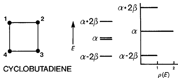
Fig. 6. The cyclobutadiene molecule (left); to the right are the four roots of equation (6), the electron energy levels are expressed in the usual form (centre) and in a density-of-states form (right).
