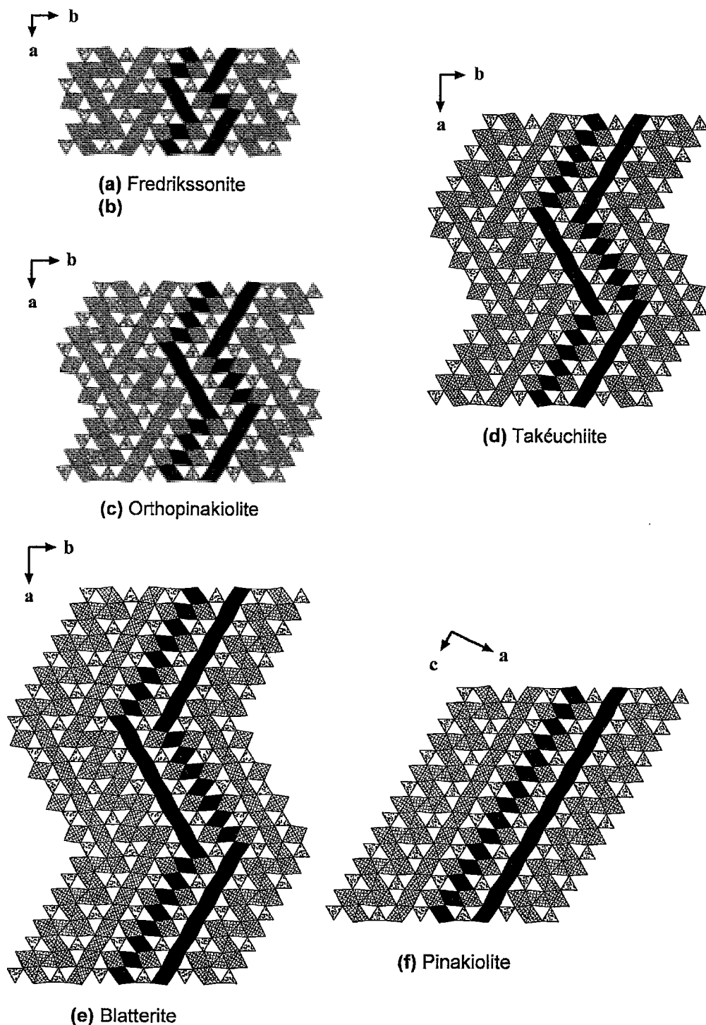
FIG. 8. Polyhedral representations of the \text{Mn}^{3+} zigzag borates viewed down [001] ([010] for pinakiolite): (a) fredrikssonite (ludwigite-type), (b) hypothetical Pnnm F_3C_3S_3 structure, (c) orthopinakiolite, (d) takéuchiite, (e) blatterite, and (f) pinakiolite. The legend is as in Figure 4; a neighboring pair of F and C walls have been shaded black.
