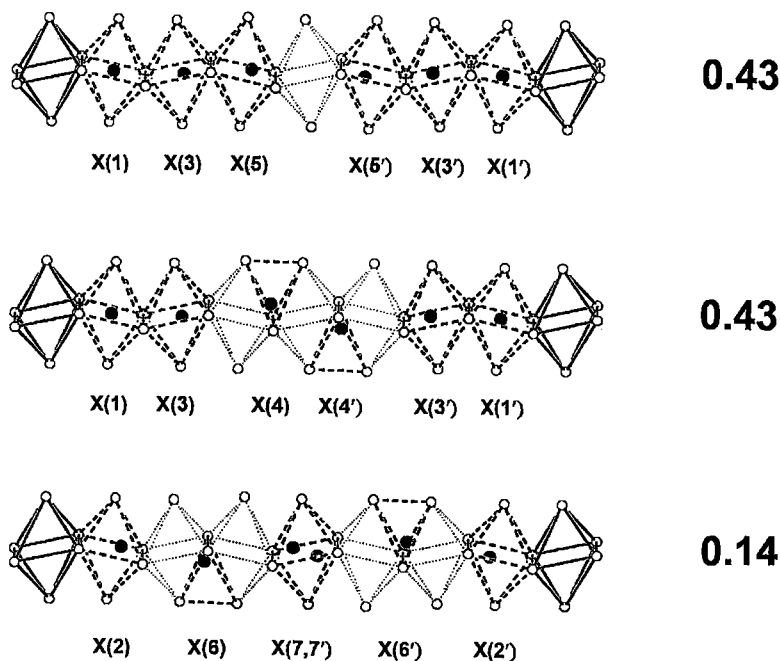
FIG. 7. Local arrangements of cations ( \text{Mn}^{2+} ) over the X sites in blatterite; the values to the right of each arrangement denote the frequency of the arrangement ( \Sigma \text{frequency} = 1 ). Note that one end of the chain of X octahedra does not have to be related to the other end by a two-fold rotation.
