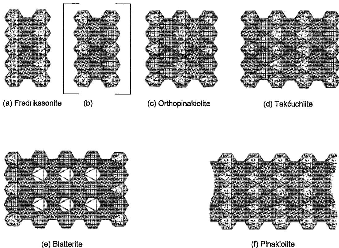
FIG. 9. The F walls in (a) fredrikssonite, (b) hypothetical Pnnm F_3C_3S_3 structure, (c) orthopinakiolite, (d) takéuchiite, (e) blatterite, and (f) pinakiolite. The legend is as in Figures 5 and 6.
