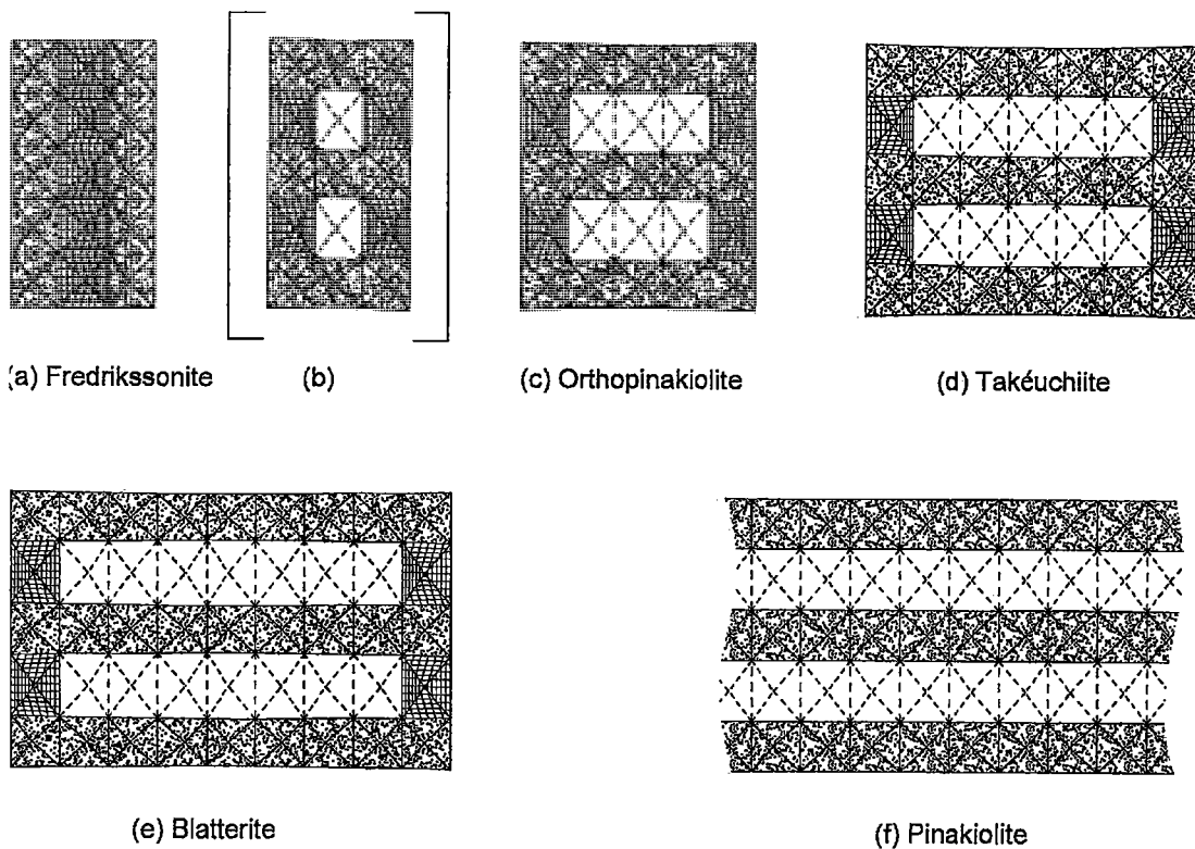
FIG. 11. The C walls in (a) fredrikssonite, (b) hypothetical Pnnm F_3C_3S_3 structure, (c) orthopinakiolite, (d) takéuchiite, (e) blatterite, and (f) pinakiolite. The legend is as in Figures 5 and 6.
