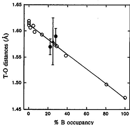
FIG. 2. The relationship between \langle T-O \rangle distances and B content; solid circle: boromuscovite ( 2M_1 ); solid triangle: boromuscovite ( 1M ); open circle: data points from Fleet (1992); line: linear regression of data points from Fleet (1992).
