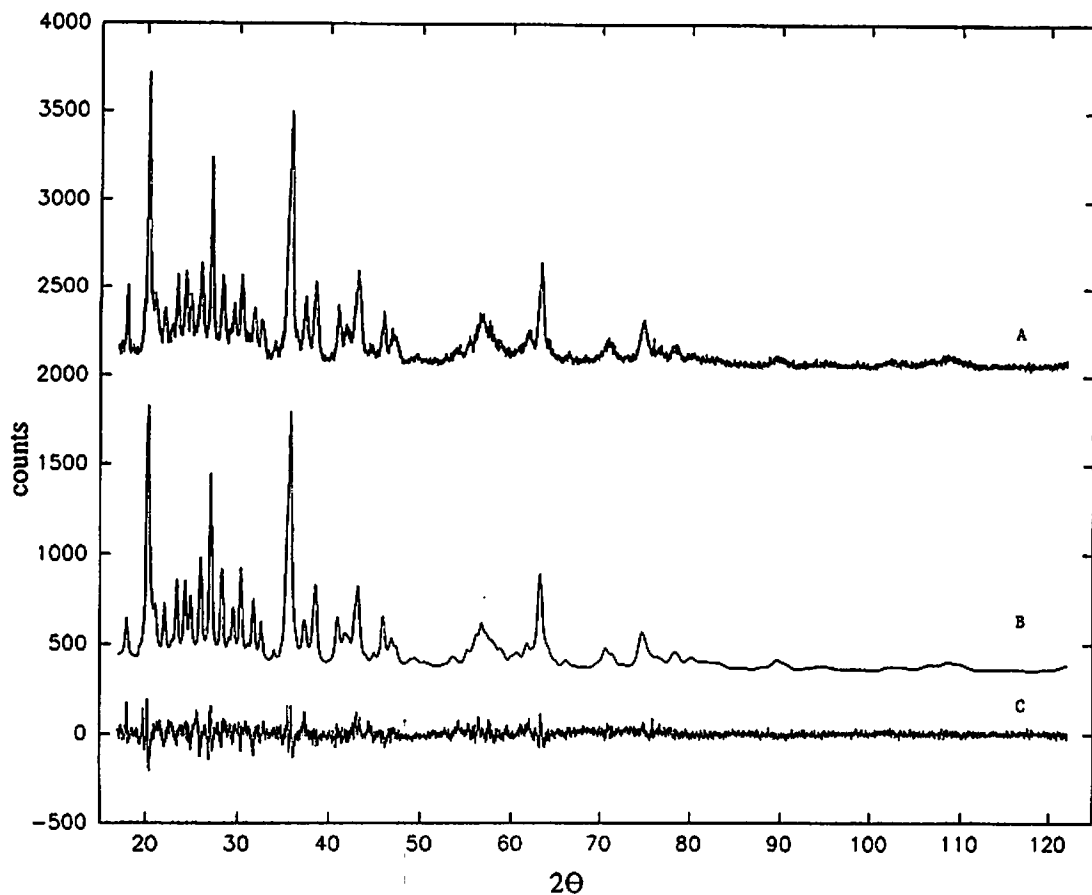
FIG. 1. A. Observed pattern. B. Calculated pattern. C. Difference between the two.
